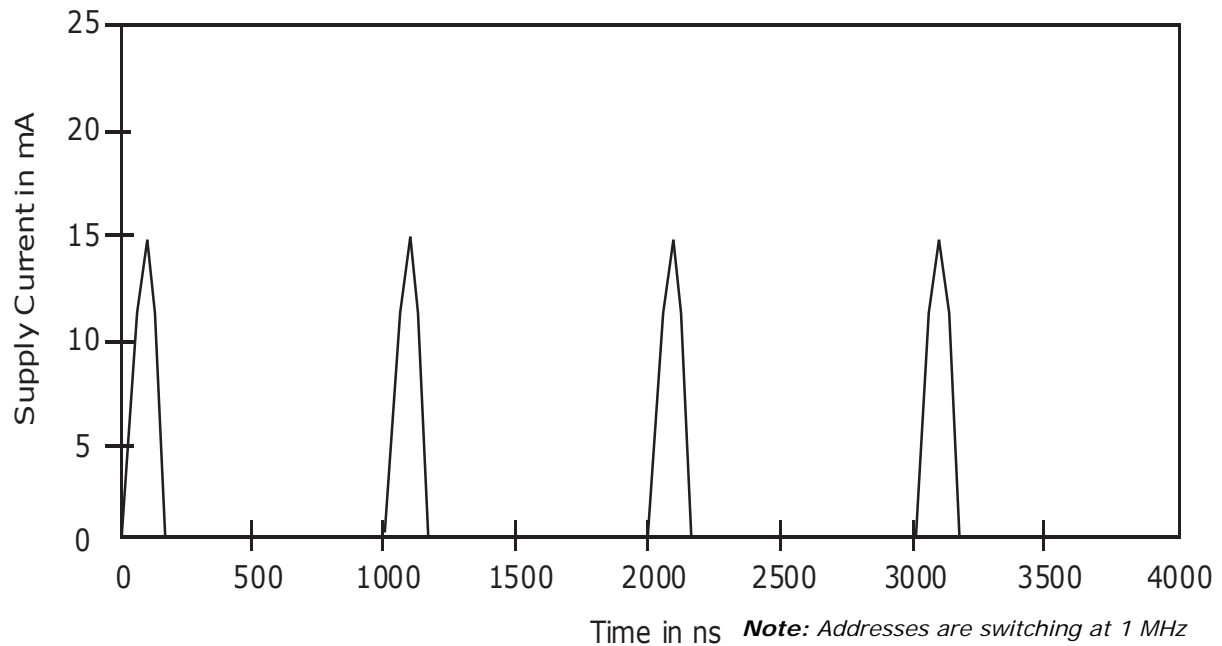
Figure 10. I_{CCI} Current vs. Time (Showing Active and Automz)
