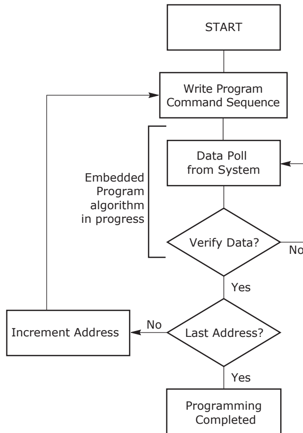
Figure 4. Program Operation
