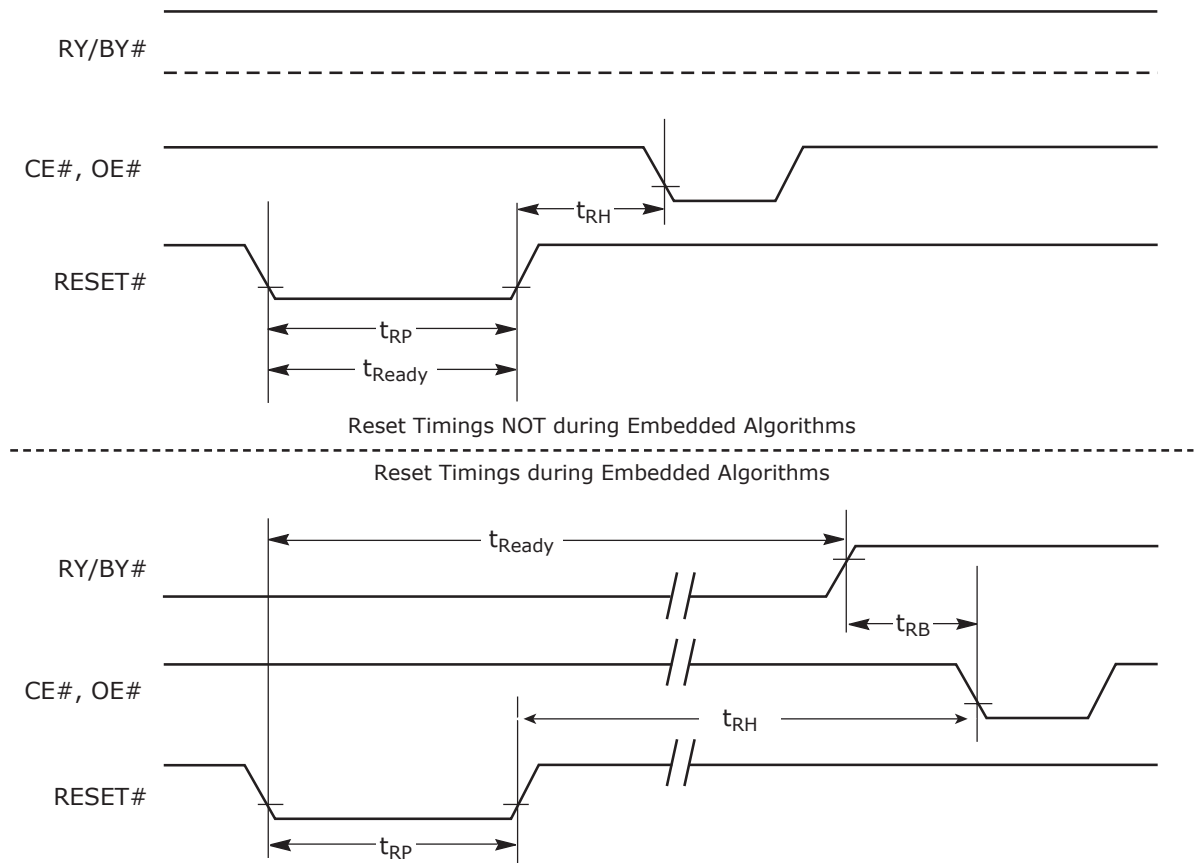
Figure I5. RESET# Timings
