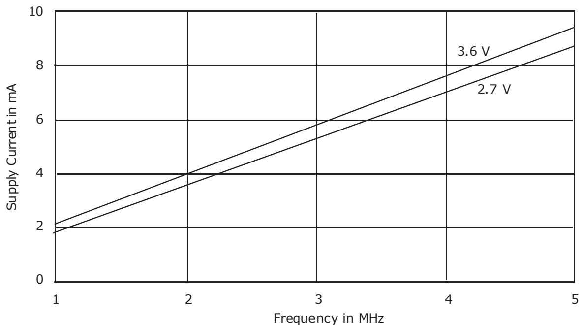
Figure II. Typical I_{CCI} vs. Frequency
