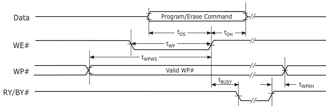
Figure 18.7 WP# Timing
