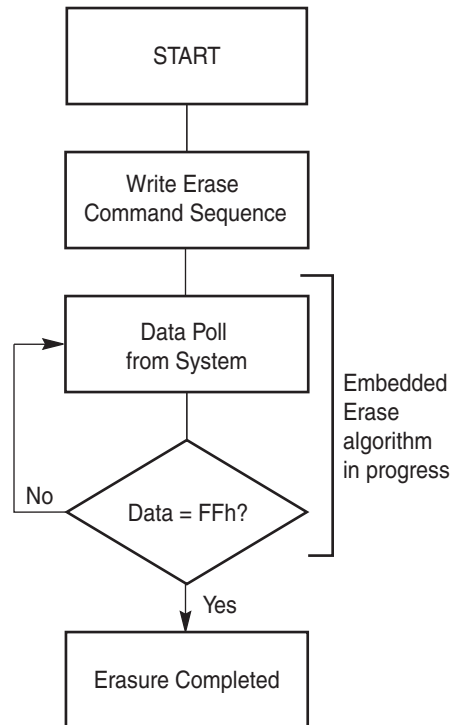
Figure 8.6 Erase Operation
