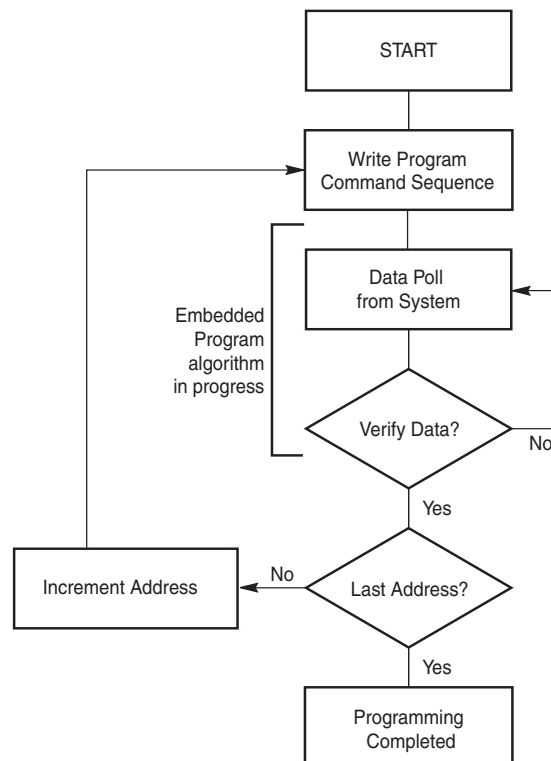
Figure 8.5 Program Operation
