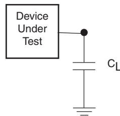
Figure 16.2 Test Setup
