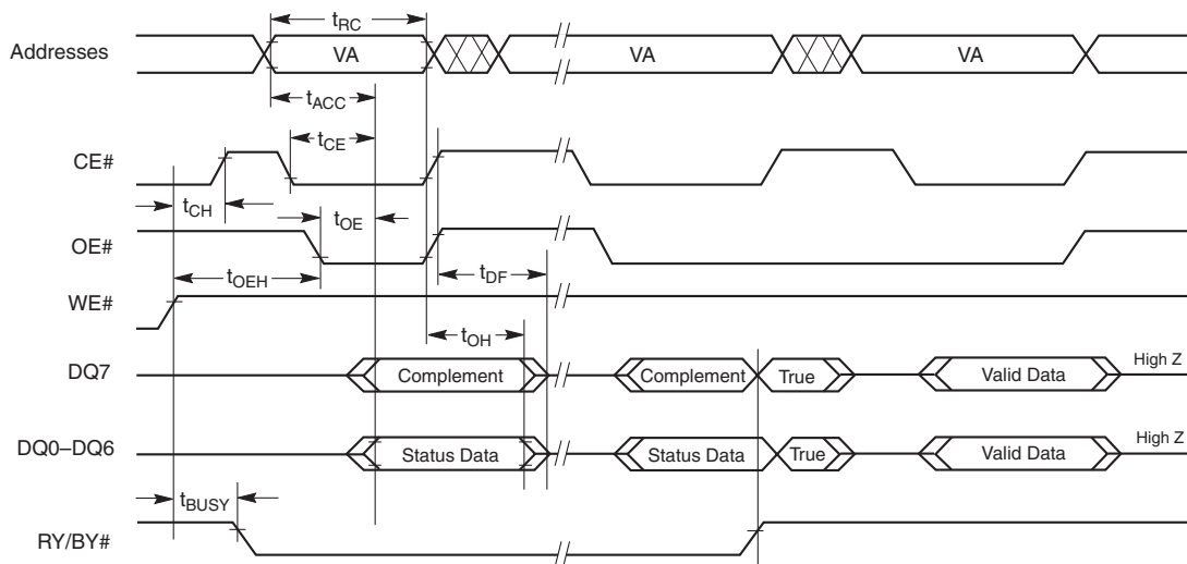
Figure 17.14 Data# Polling Timings (During Embedded Algorithms)
