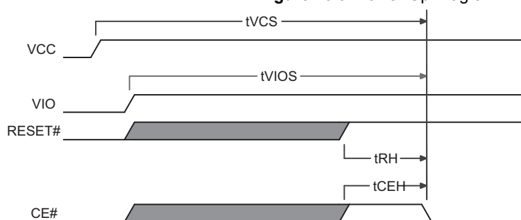
Figure 16.3 Power-Up Diagram
