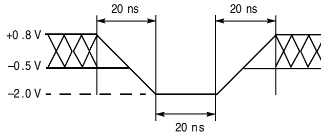
Figure 14.3 Maximum Negative Overshoot Waveform
