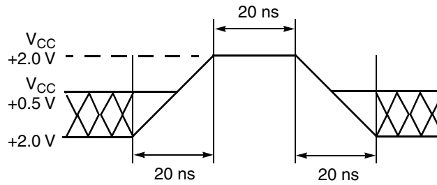
Figure 14.4 Maximum Positive Overshoot Waveform
