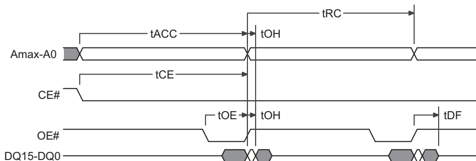
Figure 17.3 Back to Back Read Operation ( t_{RC} ) Timing Diagram
