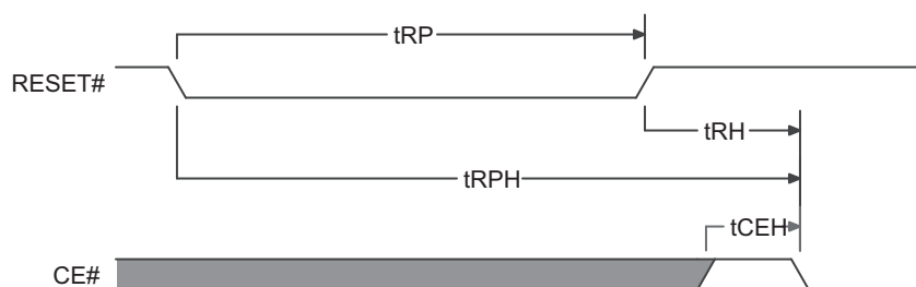
Figure 16.4 Hardware Reset
