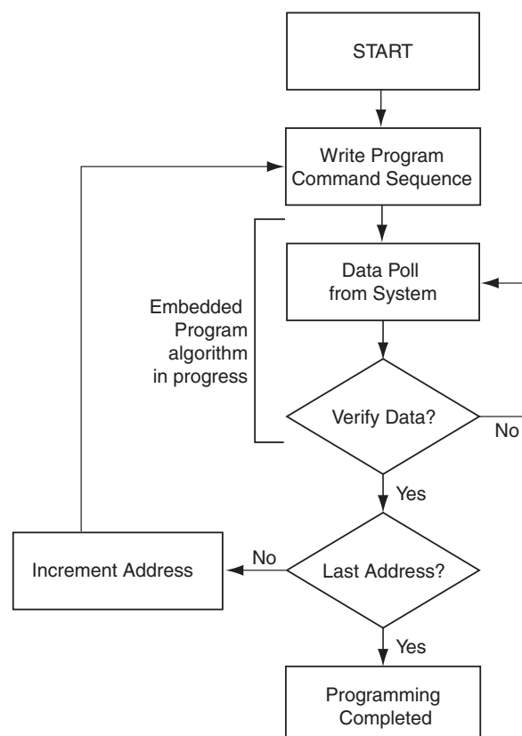
Figure 10.2 Program Operation
