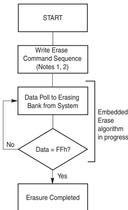
Figure 10.4 Erase Operation
