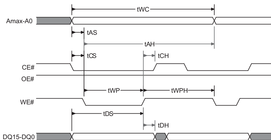
Figure 11.8 Back to Back Write Operation Timing Diagram
