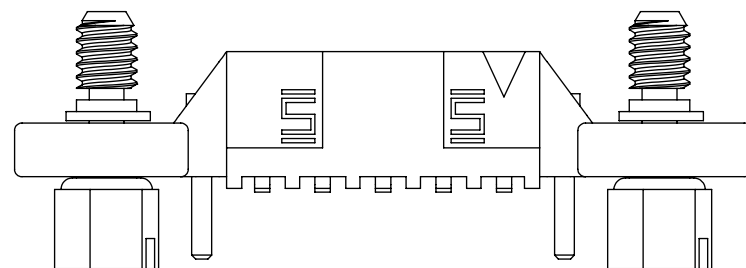
FIG 5 S2M-105-02-X-D-SD SHOWN (SAME AS FIG 4, EXCEPT AS SHOWN) (NOT RELEASED FOR PRODUCTION)
