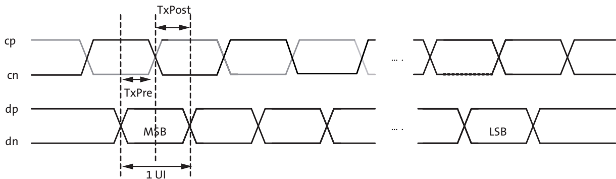
Figure 10: Timing Diagram
