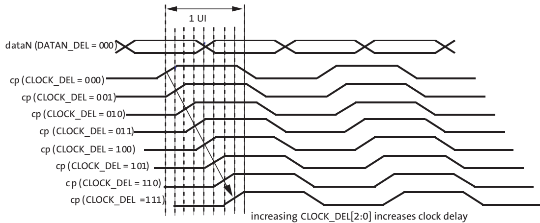
Figure 12: Delaying the Clock with Respect to Data
