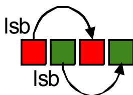
Figure 23: Horizontal Binning in the AR0141CS Sensor
