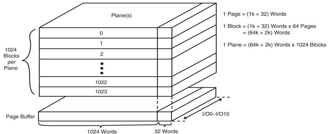
Figure 1.8 Array Organization — S34MS01G2 (x16)
