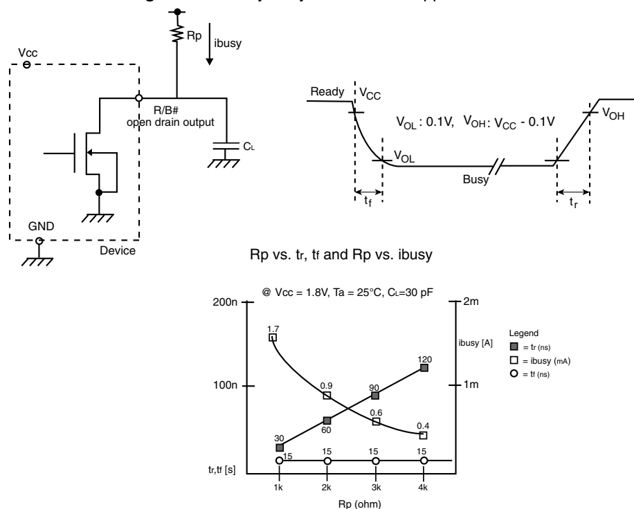
Figure 4.1 Ready/Busy Pin Electrical Application
