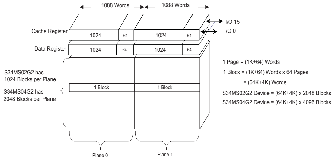
Array Organization (x16)
