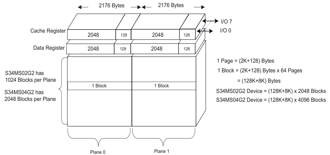
Array Organization (x8)
