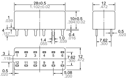
External dimensions
