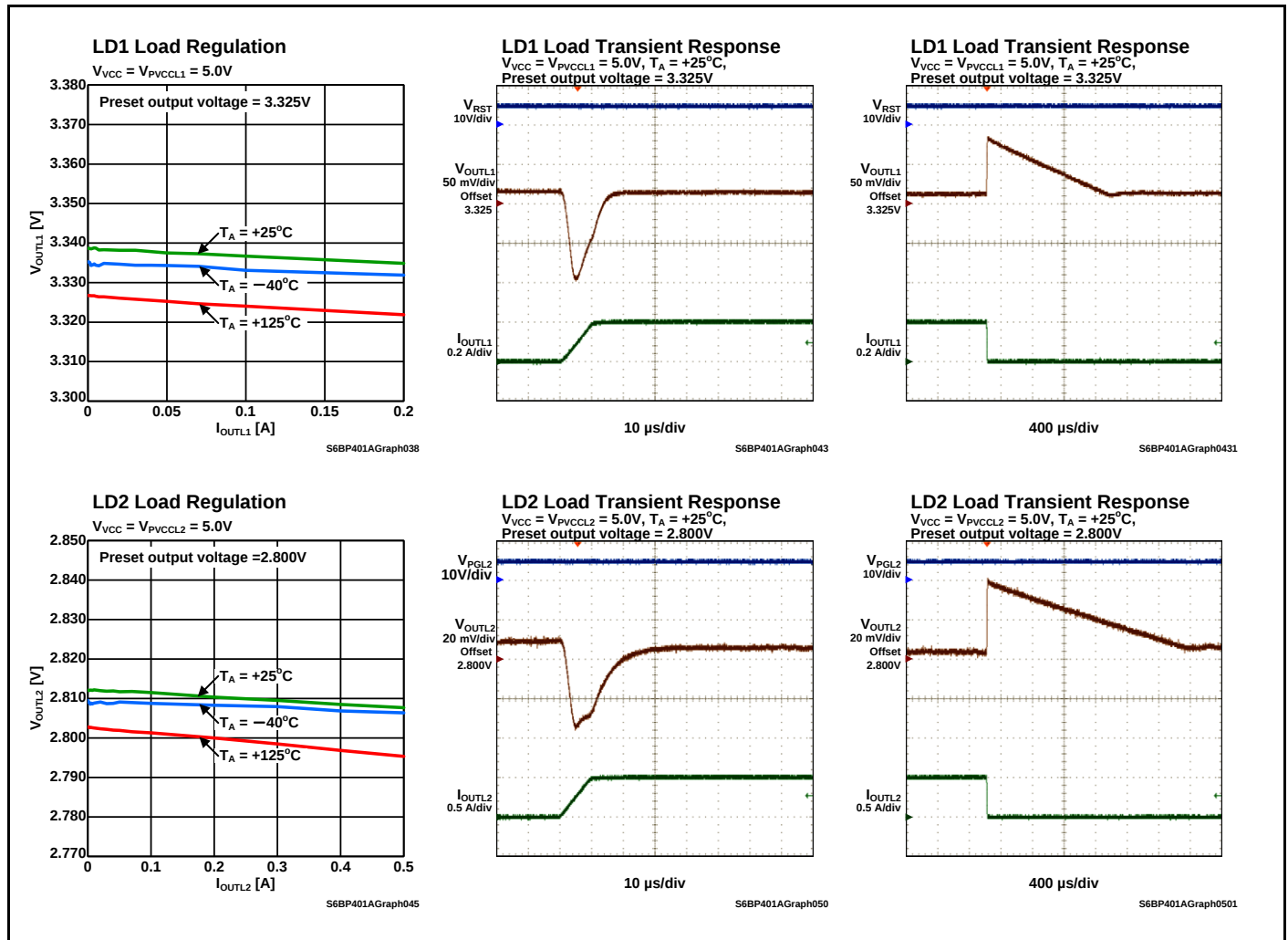
Figure 13-2 LDO regulator
