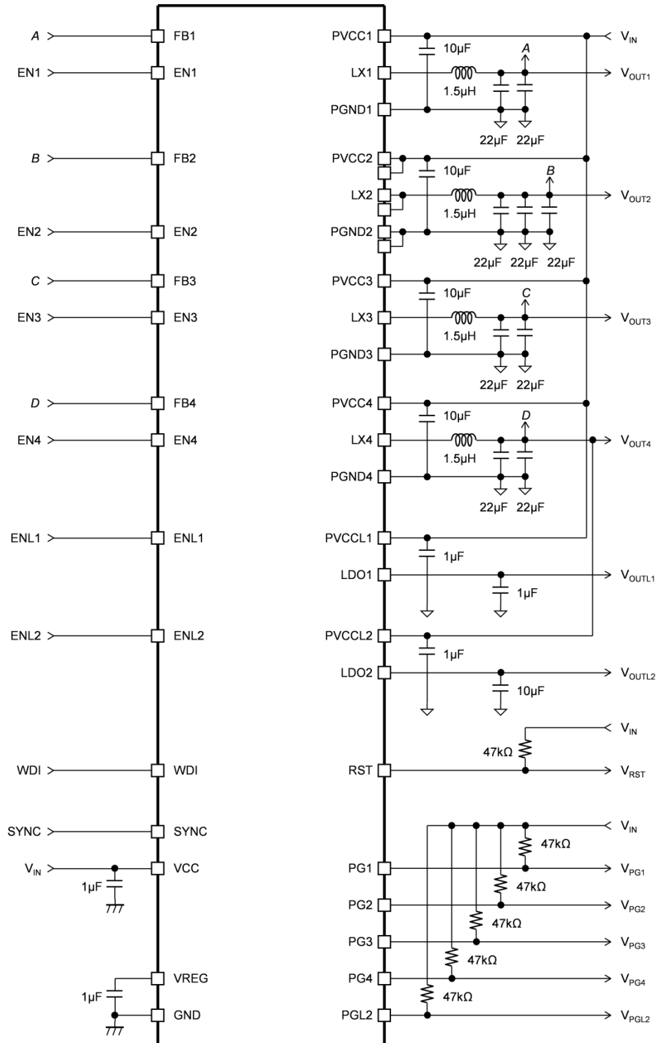
Figure 1-1 Typical Application
