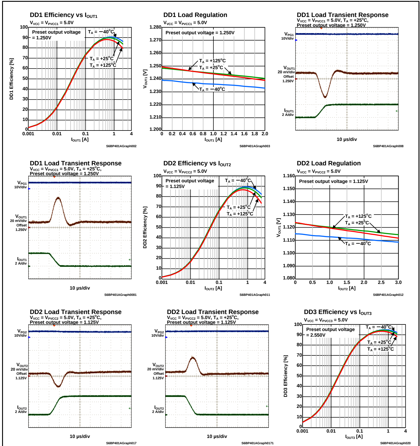
Figure 13-1 DC/DC Converter
