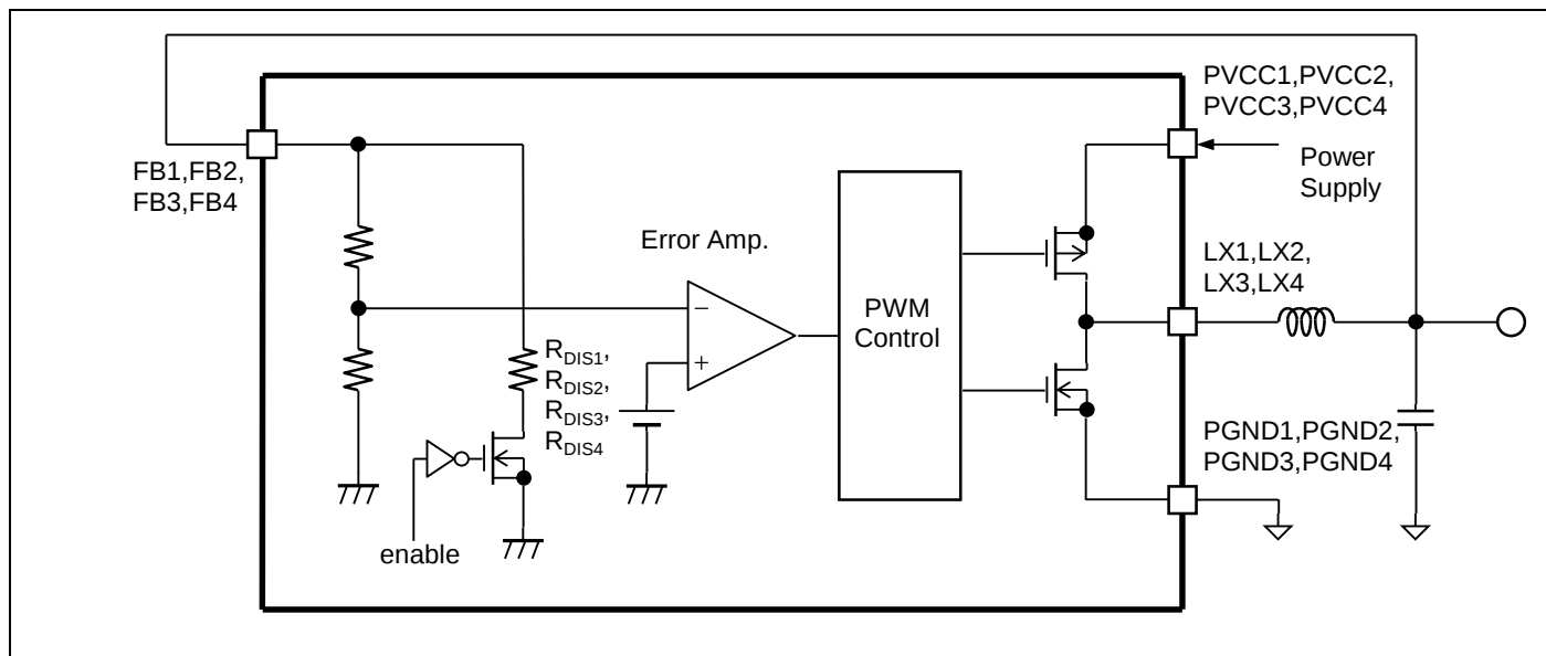
Figure 10-7 Discharge Diagram (DC/DC Converter)
