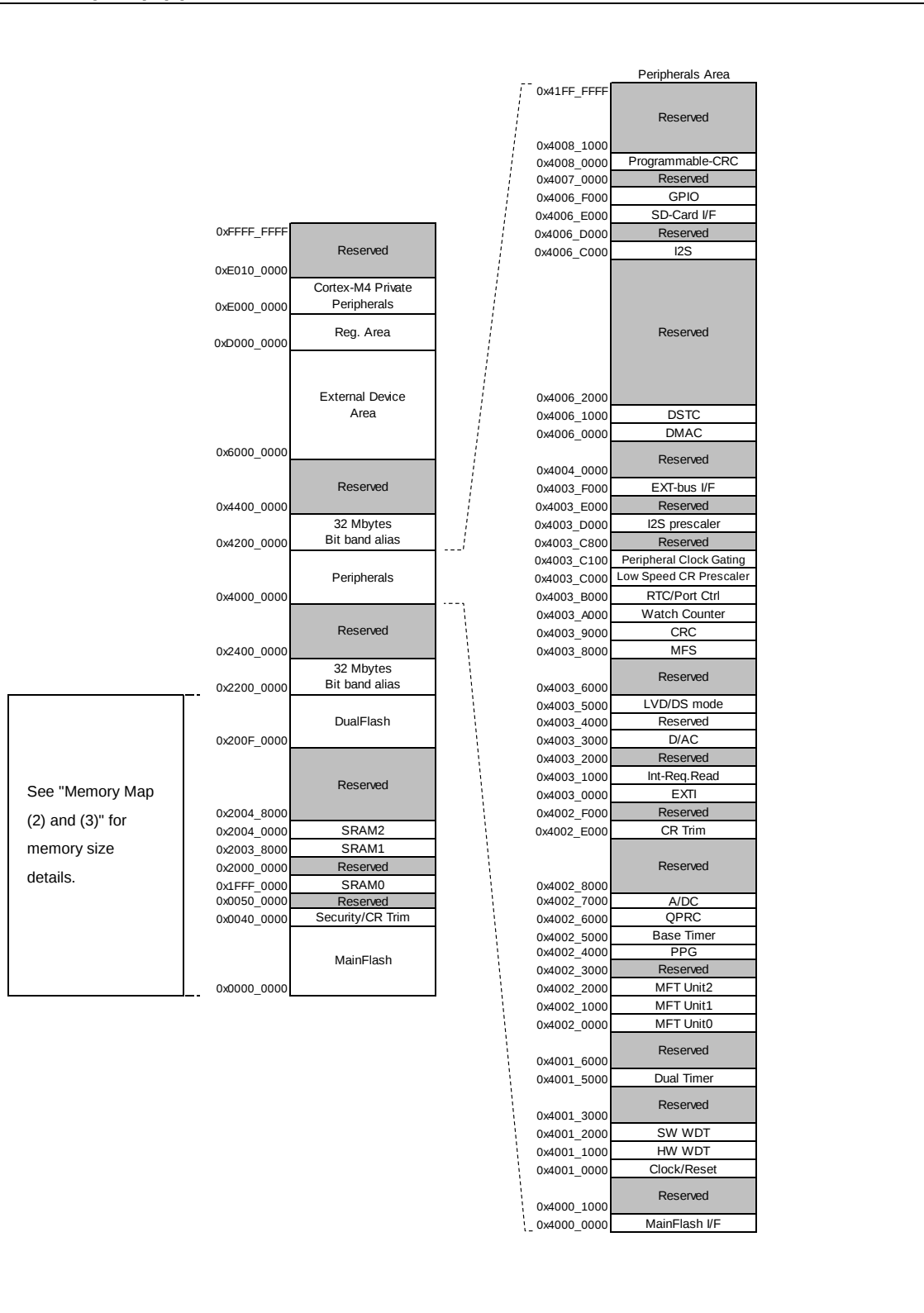
Memory Map (1)
