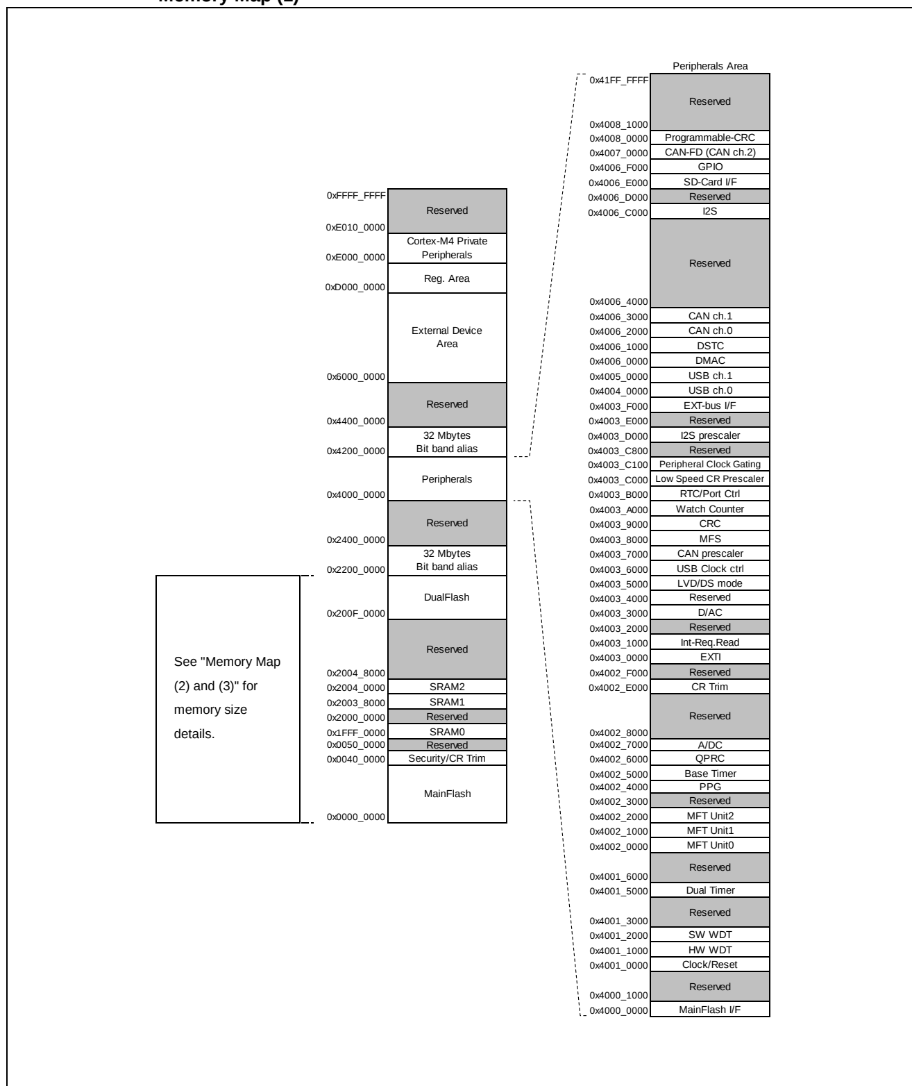
Memory Map (1)
