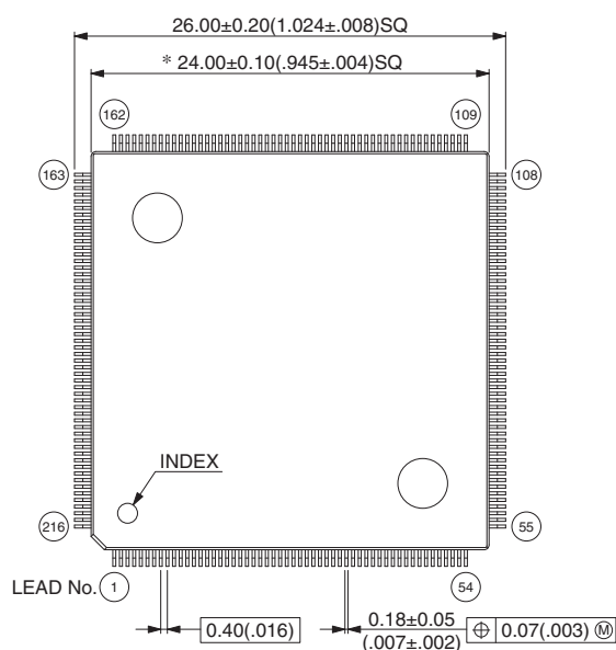
216-pin plastic LQFP (FPT-216P-M01)
