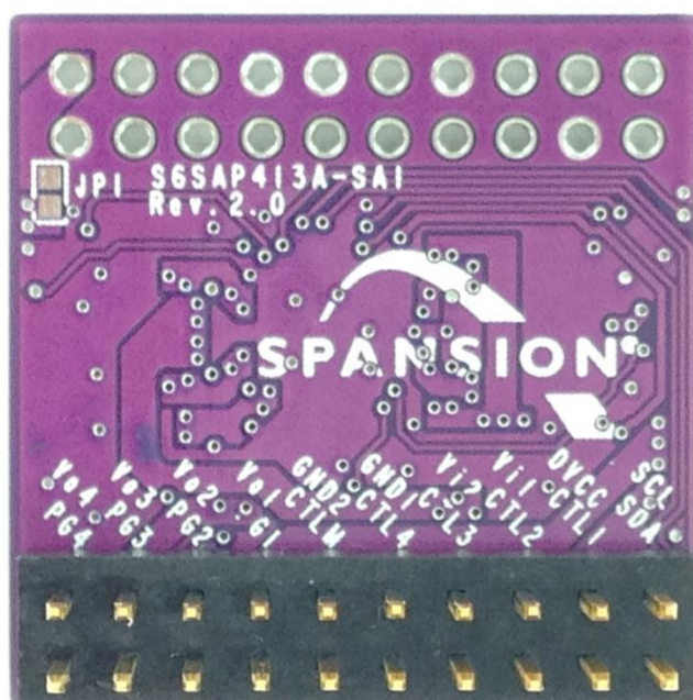
Figure8-2 Picture (Back)
