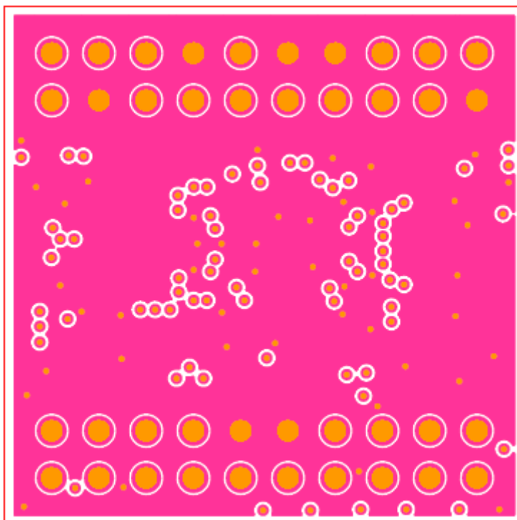
Figure5-4 Wiring Layout (Layer 2)
