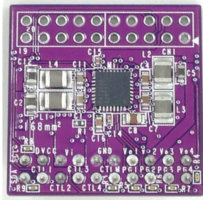
Figure8-2 Picture (Back)
