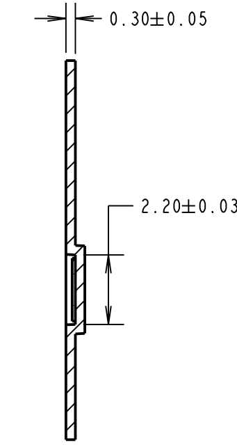
SECTION Y-Y
