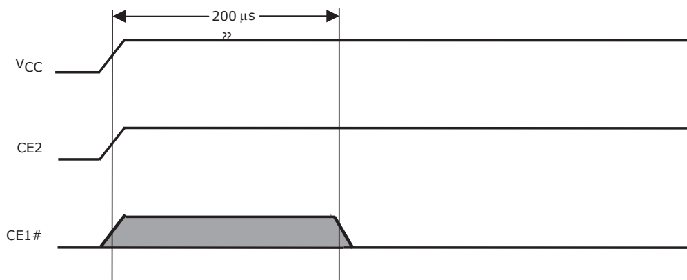
Figure 41. Power-up Mode
