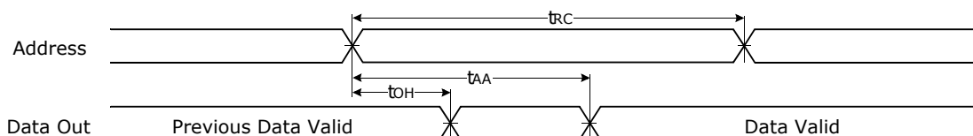
Figure 73. Timing Waveform of Read Cycle(I) (Address Controlled, CS1# = OE# = V IL , CS2 = WE# = V IH , UB# and/or LB# = V IL )
