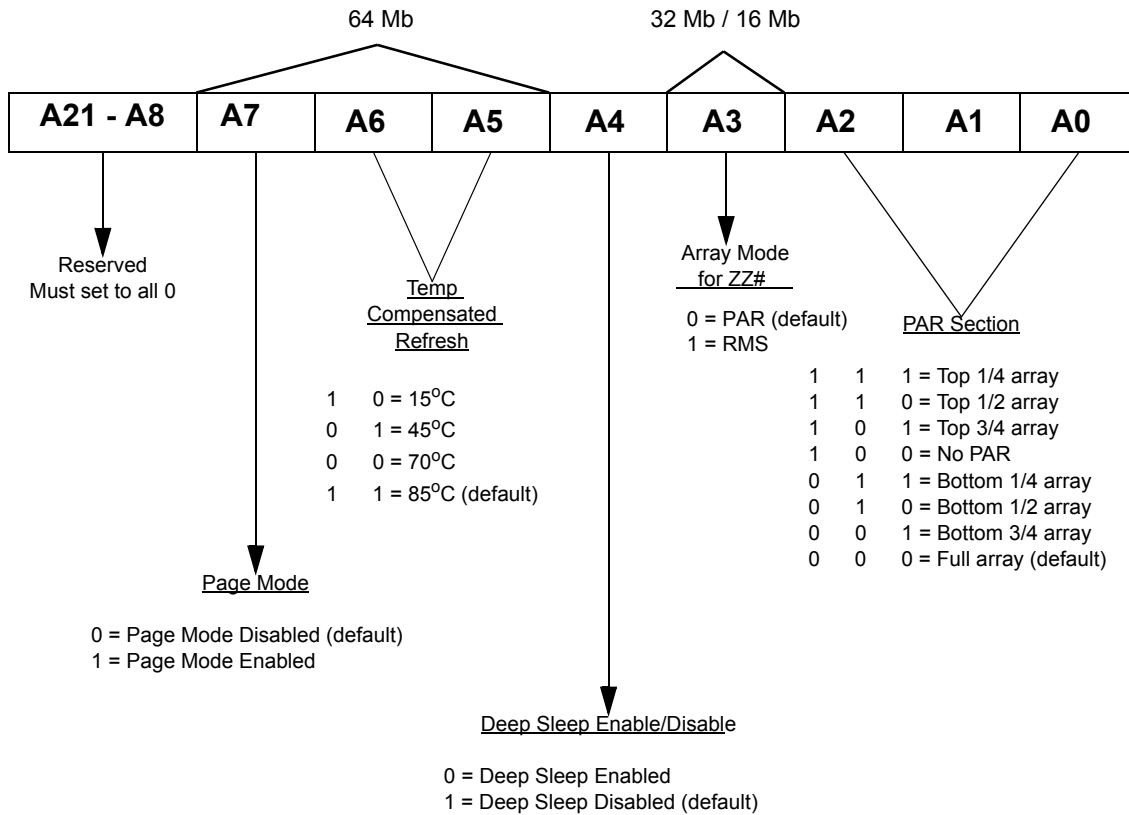
Figure 86. Mode Register
