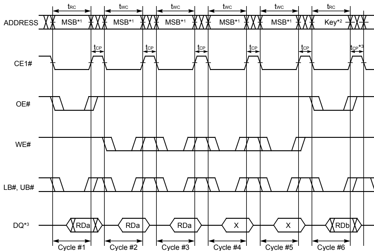
Figure 7I. Power Down Program Timing (for 32M/64M Only)
