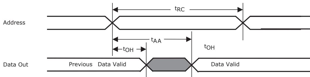
Figure 35. Read Cycle I—Addressed Controlled
