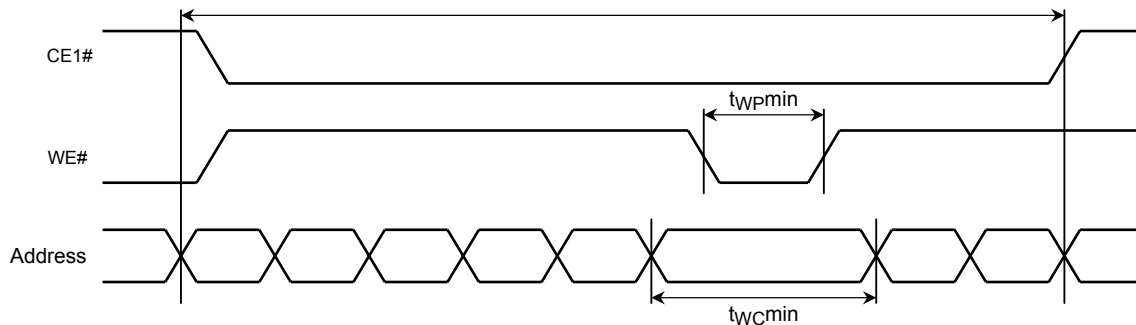
Figure 50. Write
