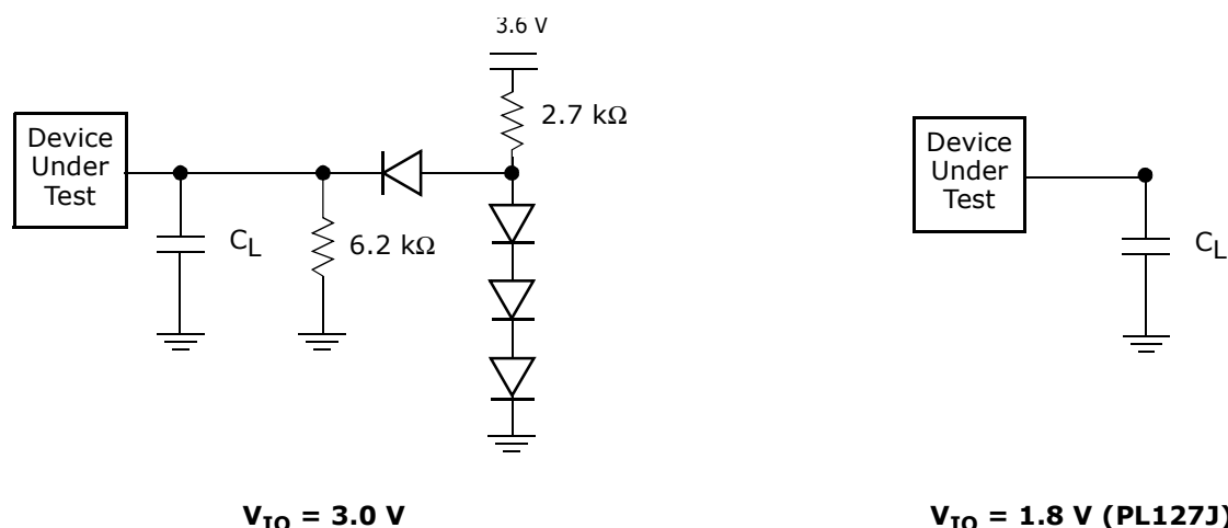
Figure 9. Test Setups
