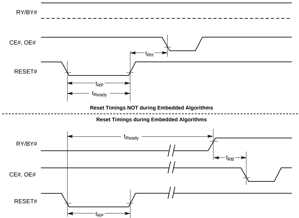
Figure I3. Reset Timings
