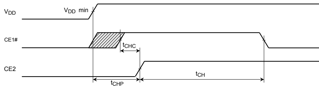
Figure 48. Power-on Timing
