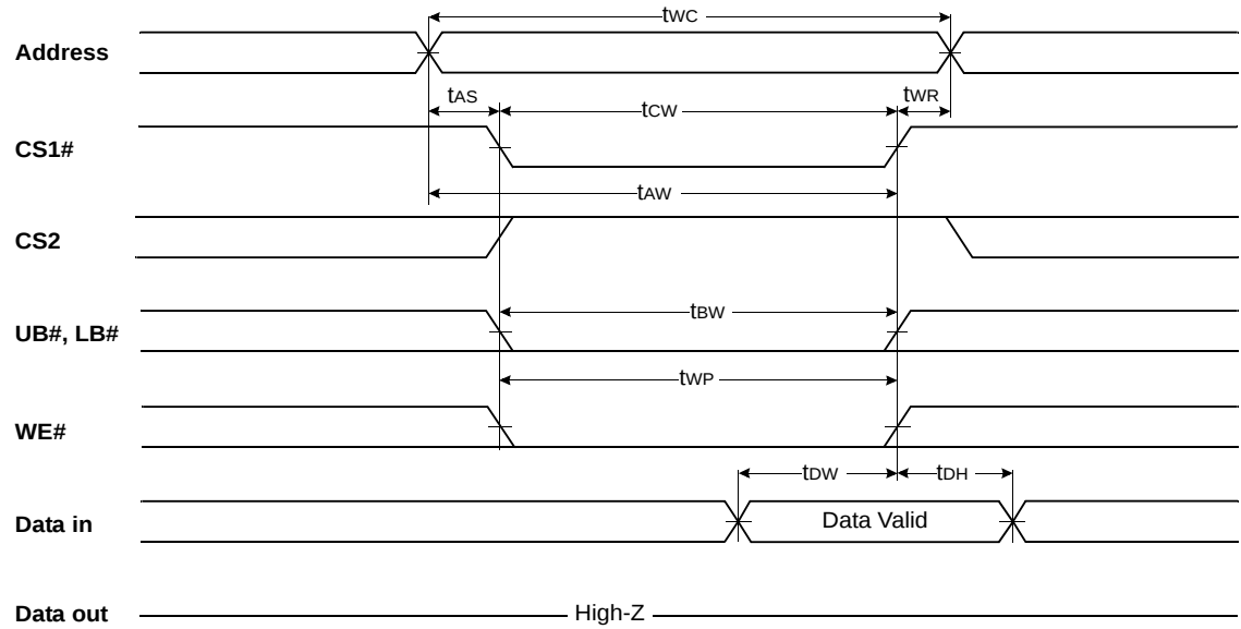
Figure 32. Write Cycle #2 (CS1# Controlled)
