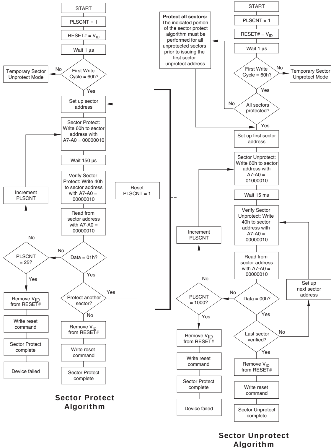
Figure 1. In-System Sector Protection/Sector Unprotection Algorithms
