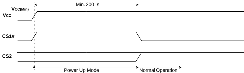
Figure 25. Power Up I (CS1# Controlled)
