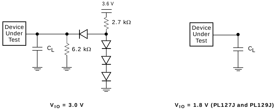
Figure 9. Test Setups
