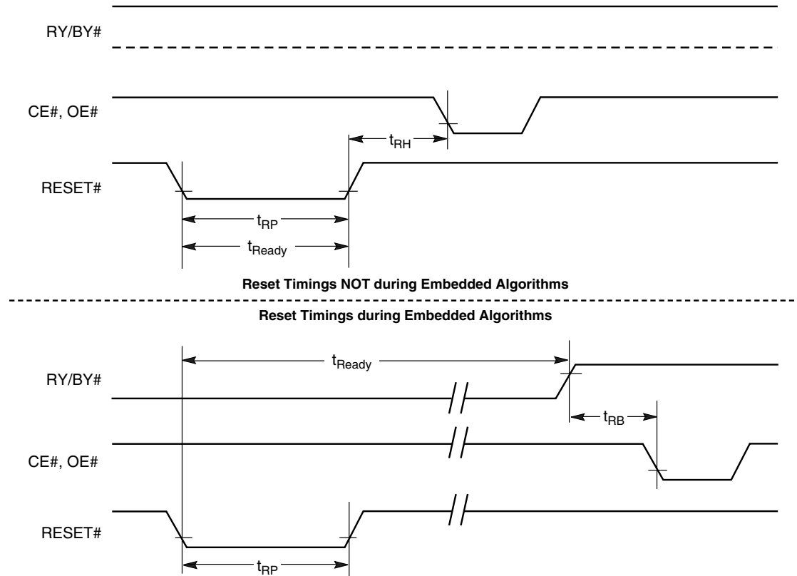
Figure I3. Reset Timings
