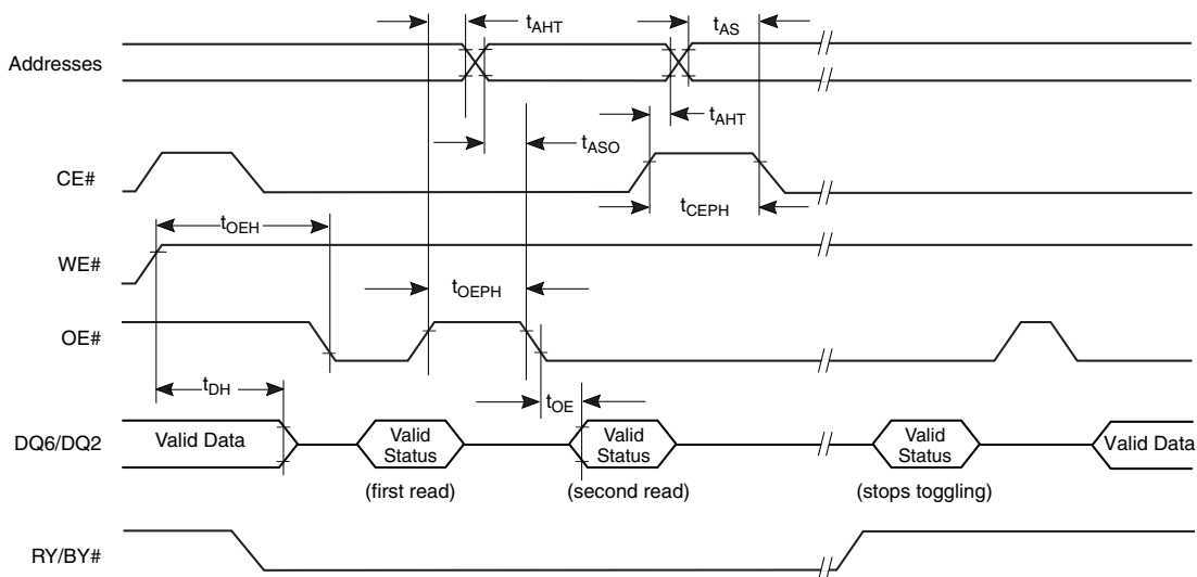
Figure I8. Data# Polling Timings (During Embedded Algorithms)
