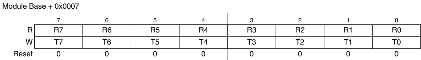
Figure 20-13. SCI Data Registers (SCIDRL)
