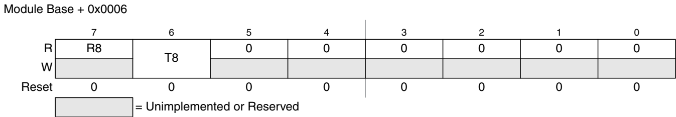
Figure 20-12. SCI Data Registers (SCIDRH)
