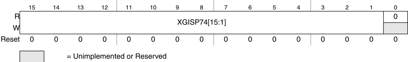
Figure 10-7. XGATE Initial Stack Pointer for Interrupt Priorities 7 to 4 (XGISP74)
