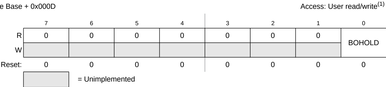
Figure 14-17. MSCAN Miscellaneous Register (CANMISC)
