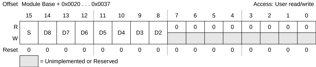
Figure 11-9. Motor Controller Duty Cycle Register x (MCDcCx) with FAST = 1
