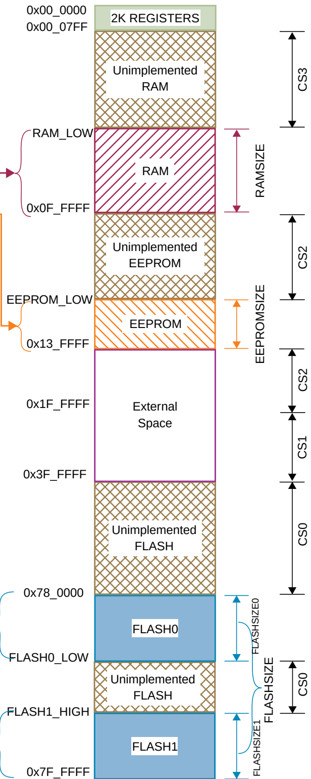
Figure 25-23. Local to Implemented Global Address Mapping (Without GPAGE)
