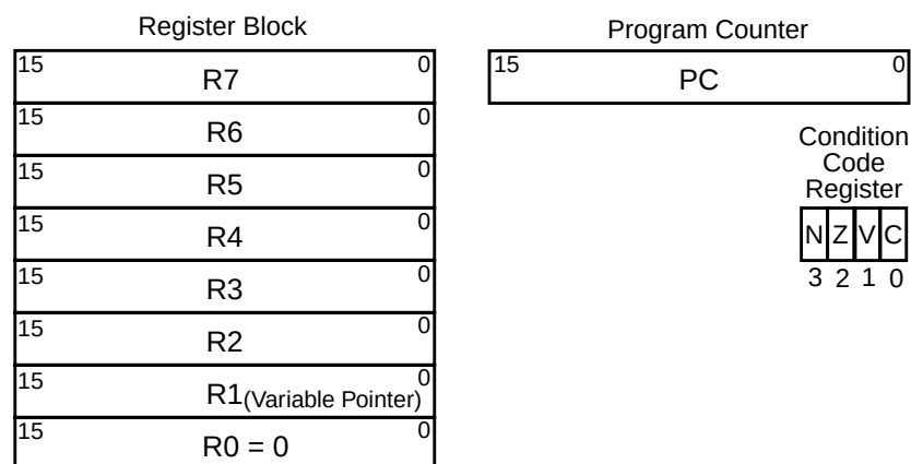
Figure 5-19. Programmer's Model
