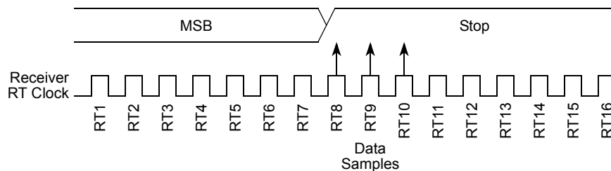
Figure 16-28. Slow Data
