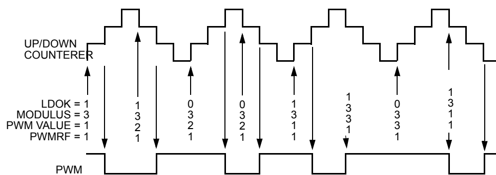
Figure 15-78. Half-Cycle Center-Aligned PWM Value Loading
