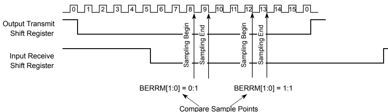
Figure 16-19. Timing Diagram Bit Error Detection
