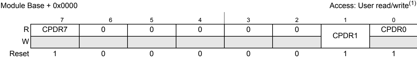
Figure 21-2. Port CP Data Register (CPDR)
