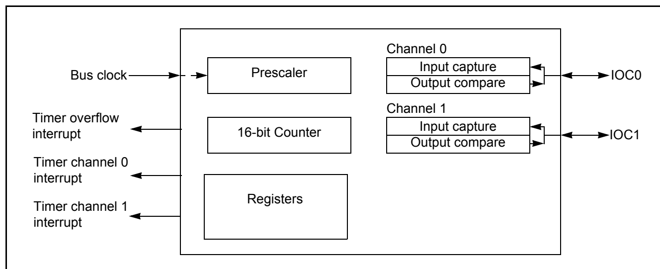
Figure 12-1. TIM16B2CV3 Block Diagram
