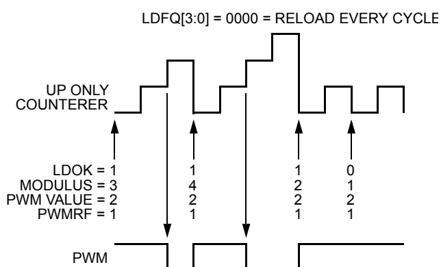
Figure 15-81. Edge-Aligned Modulus Loading
