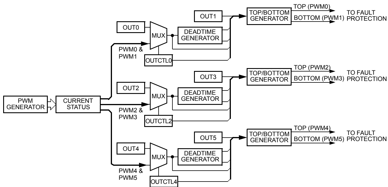
Figure 15-50. Deadtime Generators
