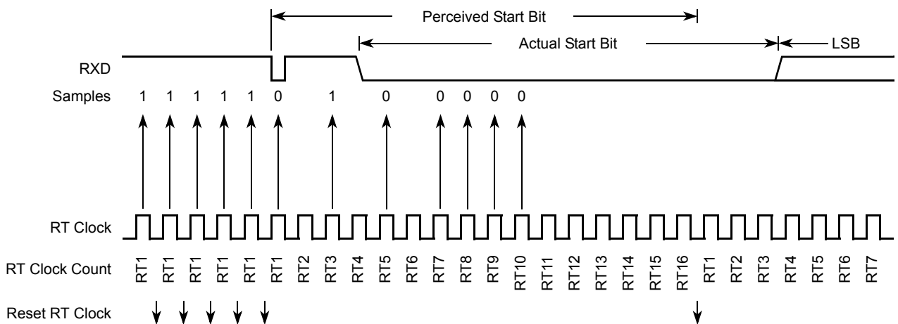
Figure 16-23. Start Bit Search Example 2
