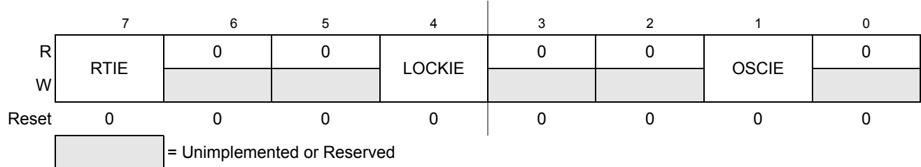
Figure 8-13. S12CPMU_UHV_V10_V6 Interrupt Enable Register (CPMUINT)
