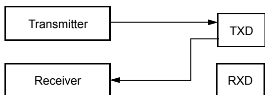
Figure 16-30. Single-Wire Operation (LOOPS = 1, RSRC = 1)
