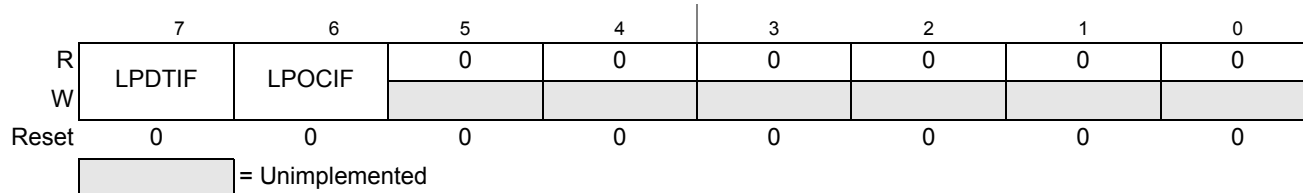
Figure 19-10. LIN Interrupt Flags Register (LPIF)
