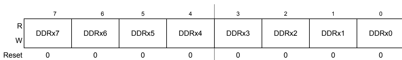
Figure 2-14. Data Direction Register
