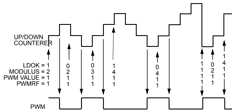
Figure 15-79. Half-Cycle Center-Aligned Modulus Loading
