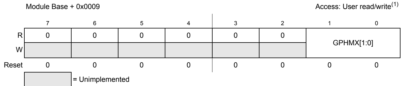
Figure 18-12. GDU Phase Mux Register (GDUPHMUX)
