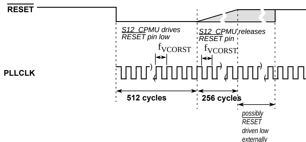
Figure 8-45. RESET Timing
