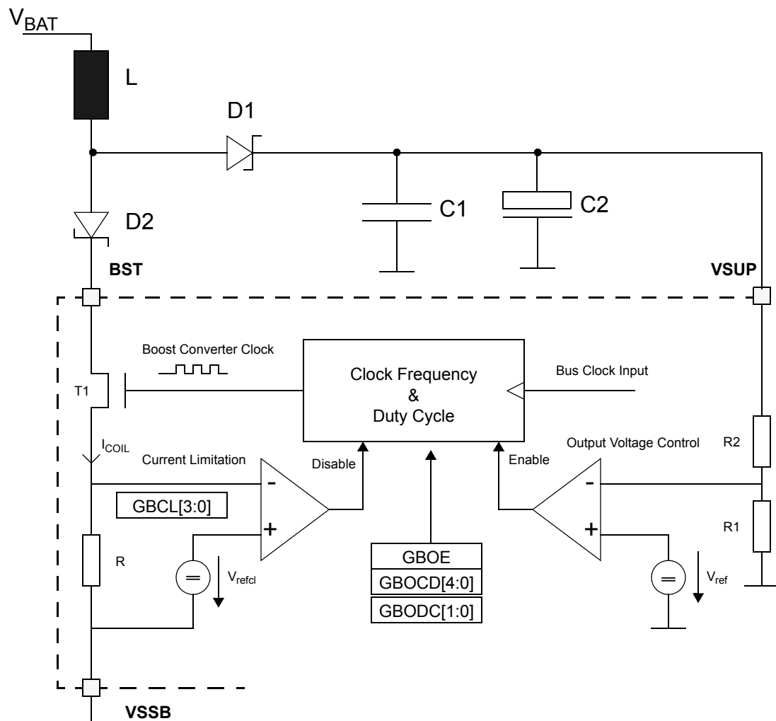
Figure 18-28. Boost Converter Option with external Components 1
