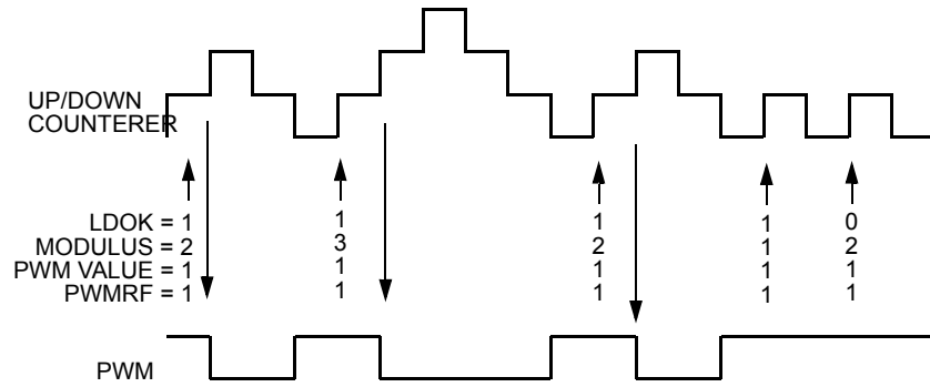
Figure 15-77. Full-Cycle Center-Aligned Modulus Loading
