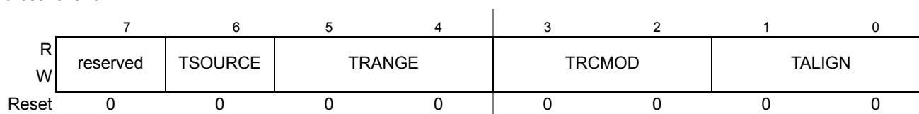
Figure 6-5. Debug Trace Control Register (DBGTCRH)
