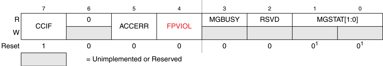
Figure 25-11. Flash Status Register (FSTAT)
