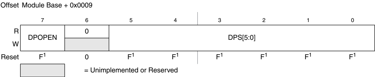
Figure 26-15. EEPROM Protection Register (EPROT)
