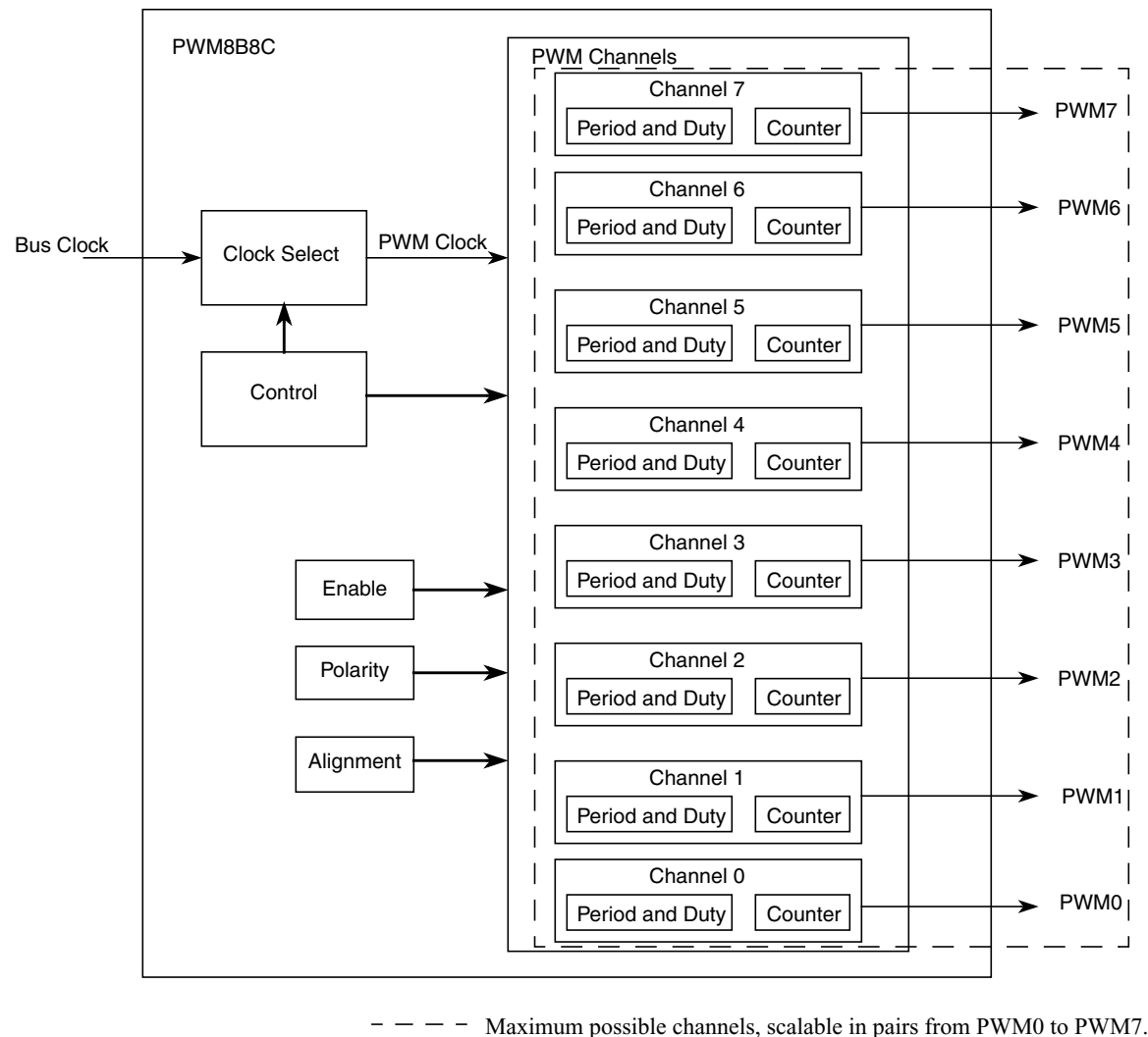
Figure 19-1. Scalable PWM Block Diagram
