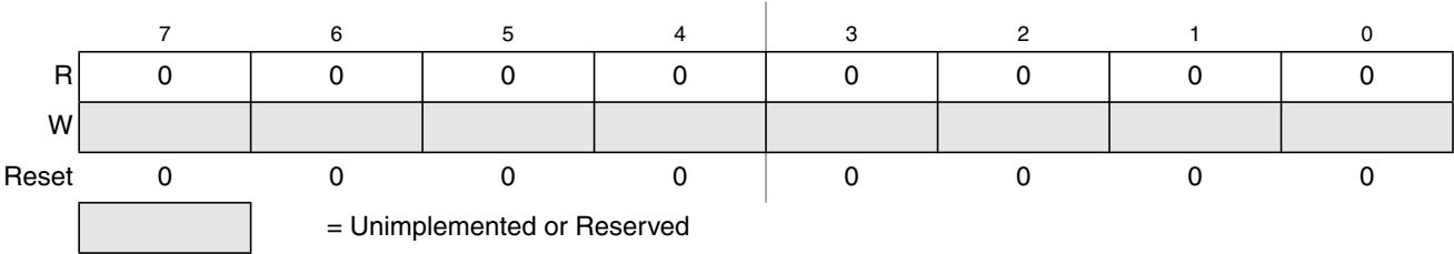
Figure 27-25. Flash Reserved7 Register (FRSV7)
