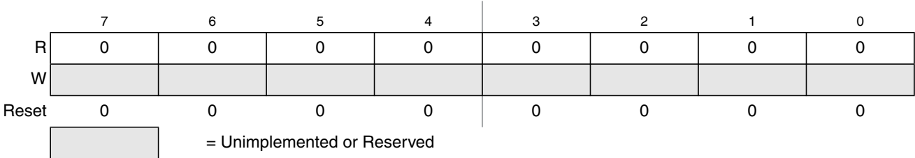
Figure 30-25. Flash Reserved7 Register (FRSV7)
