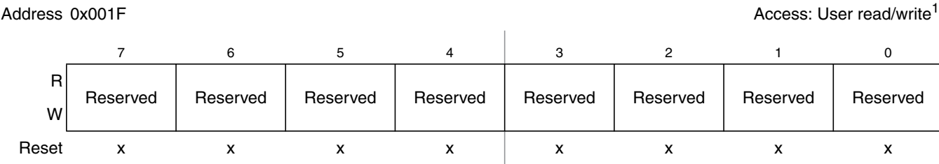
Figure 2-15. Reserved Register
