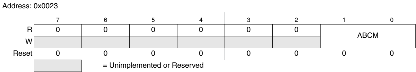
Figure 8-6. Debug Control Register2 (DBGC2)
