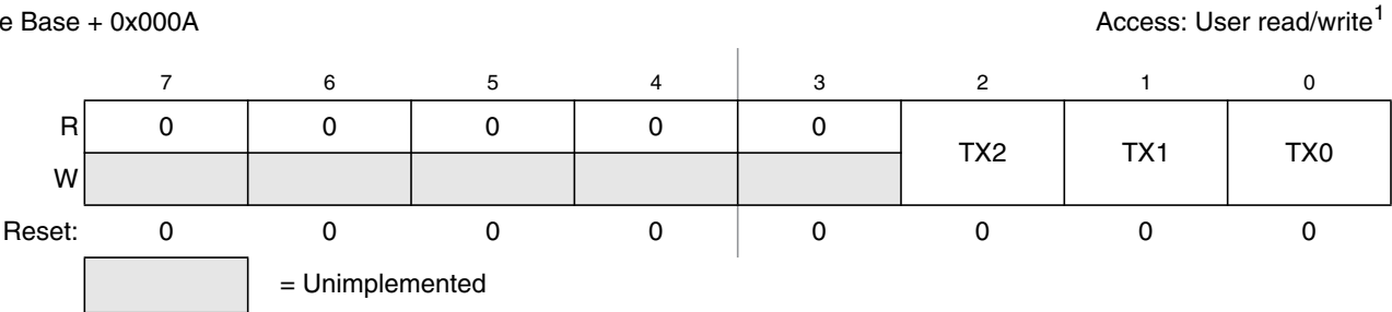
Figure 18-14. MSCAN Transmit Buffer Selection Register (CANTBSEL)
