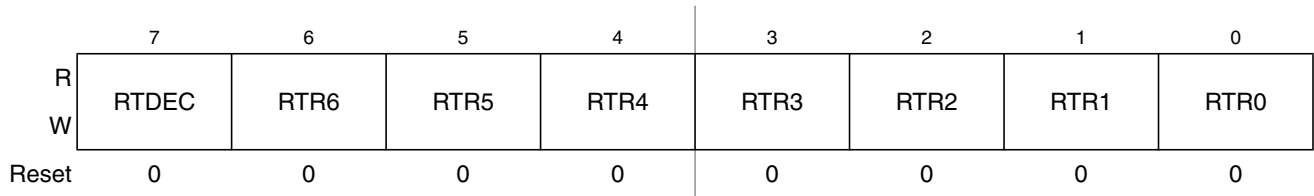
Figure 10-11. S12CPMU RTI Control Register (CPMURTI)
