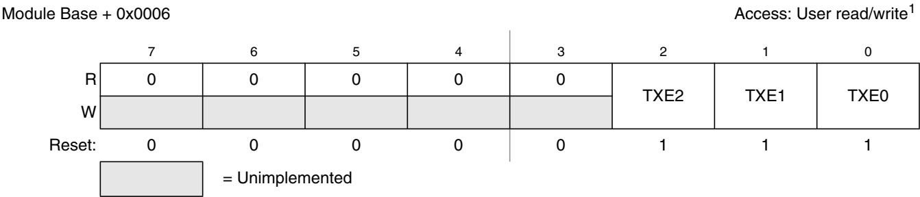
Figure 18-10. MSCAN Transmitter Flag Register (CANTFLG)
