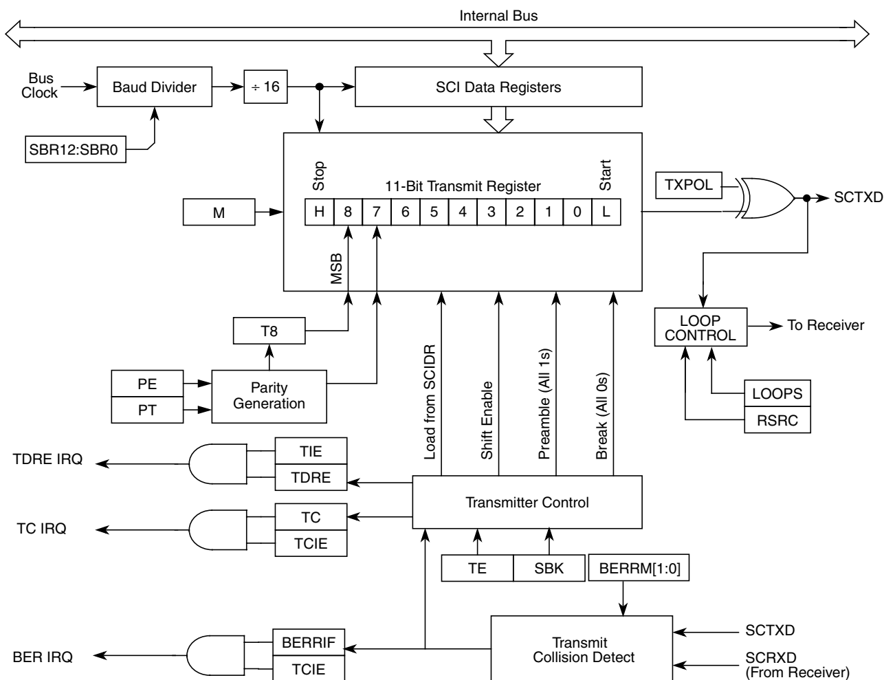
Figure 20-16. Transmitter Block Diagram
