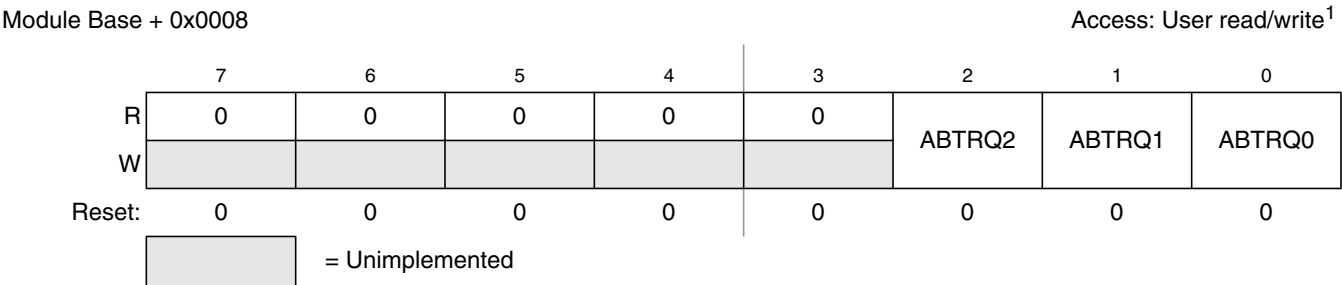
Figure 18-12. MSCAN Transmitter Message Abort Request Register (CANTARQ)
