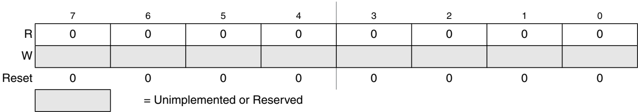
Figure 29-25. Flash Reserved7 Register (FRSV7)
