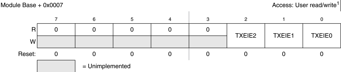
Figure 18-11. MSCAN Transmitter Interrupt Enable Register (CANTIER)
