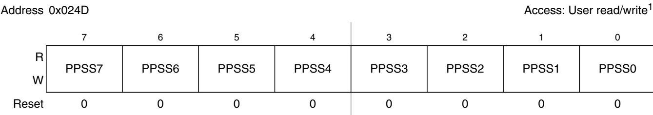
Figure 2-25. Port S Polarity Select Register (PPSS)
