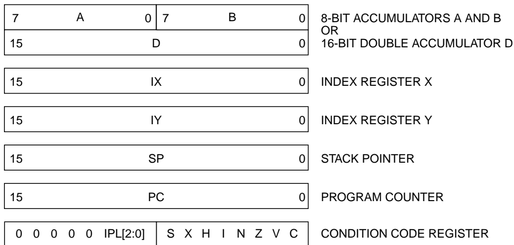
Figure 2-2. HCS12X Programming Model
