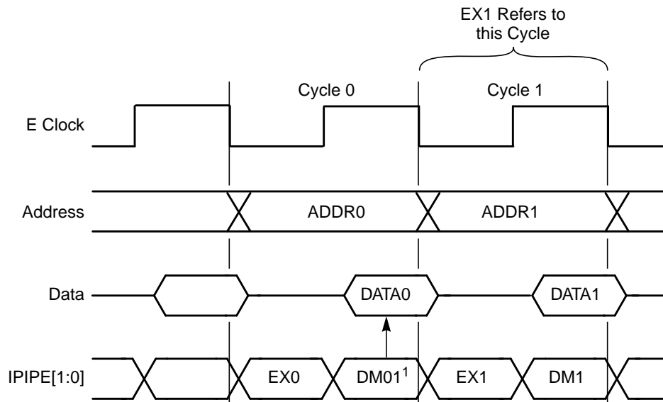
Figure 8-1. Queue Status Signal Timing (HCS12)
