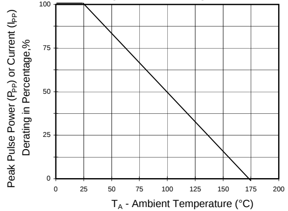
Fig.2-Power Derating Curve
