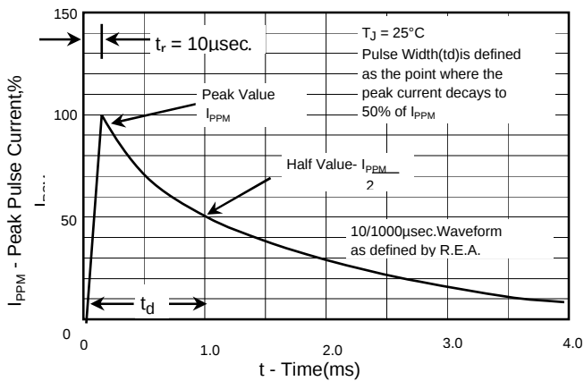
Fig.3 - Pulse Waveform
