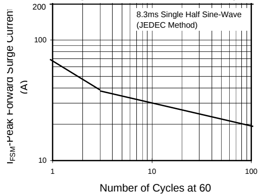
Fig.6 - Maximum Non-Repetitive Forward Surge Current Uni-Directional Only
