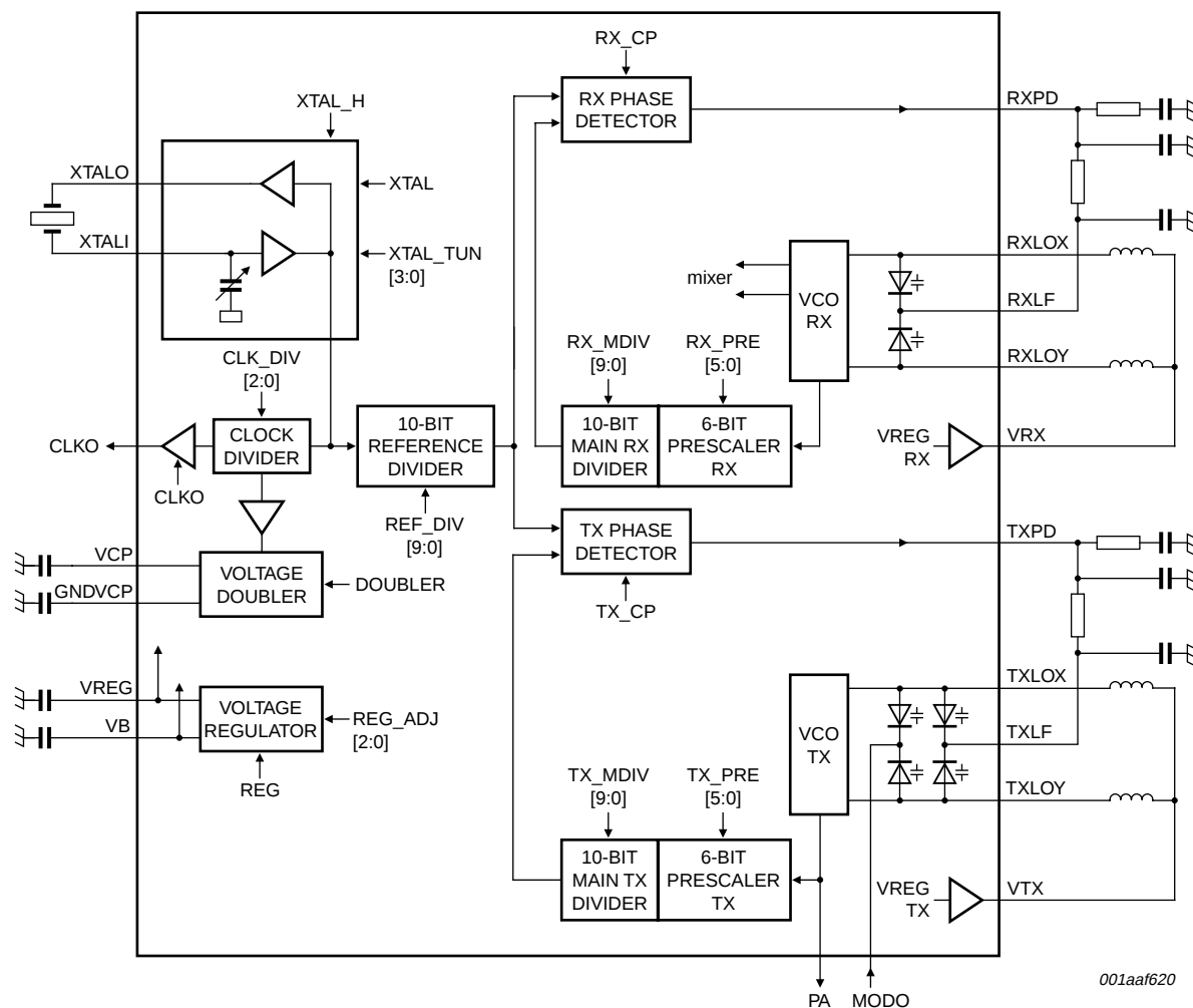
Fig 5. Synthesizer part
