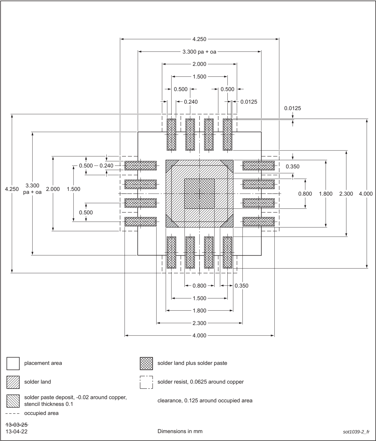
Footprint information for reflow soldering of HXQFN16 package SOT1039-2
