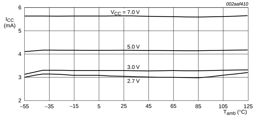
Fig 4. Supply current versus ambient temperature
