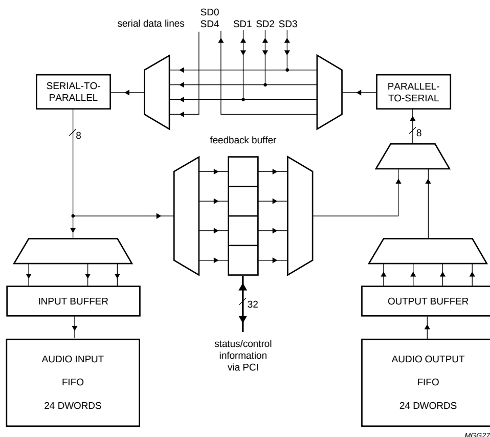
Fig.39 Audio data flow control in A1 and A2.
