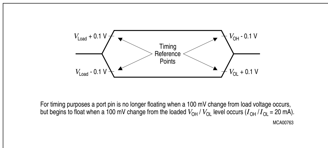
Figure 14 Float Waveforms
