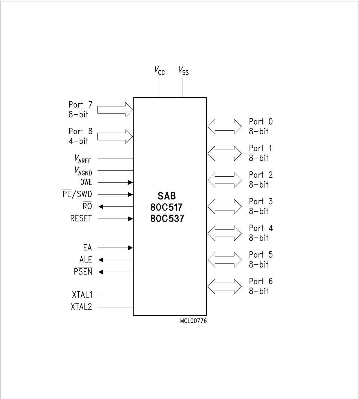
Logic Symbol
