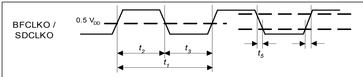
Figure 4-9 EBU Clock Output Timing
