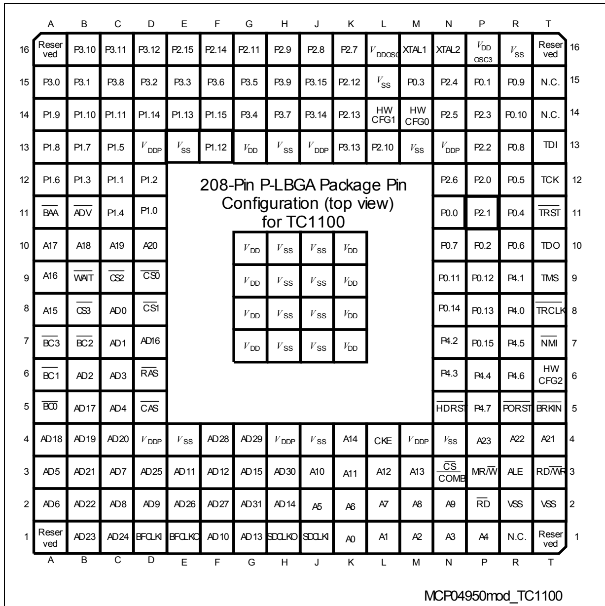
Figure 2-3 TC1100 Pins: P-BGA-208 Package (top view)
