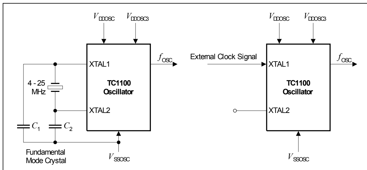
Figure 3-14 Oscillator Circuitries
