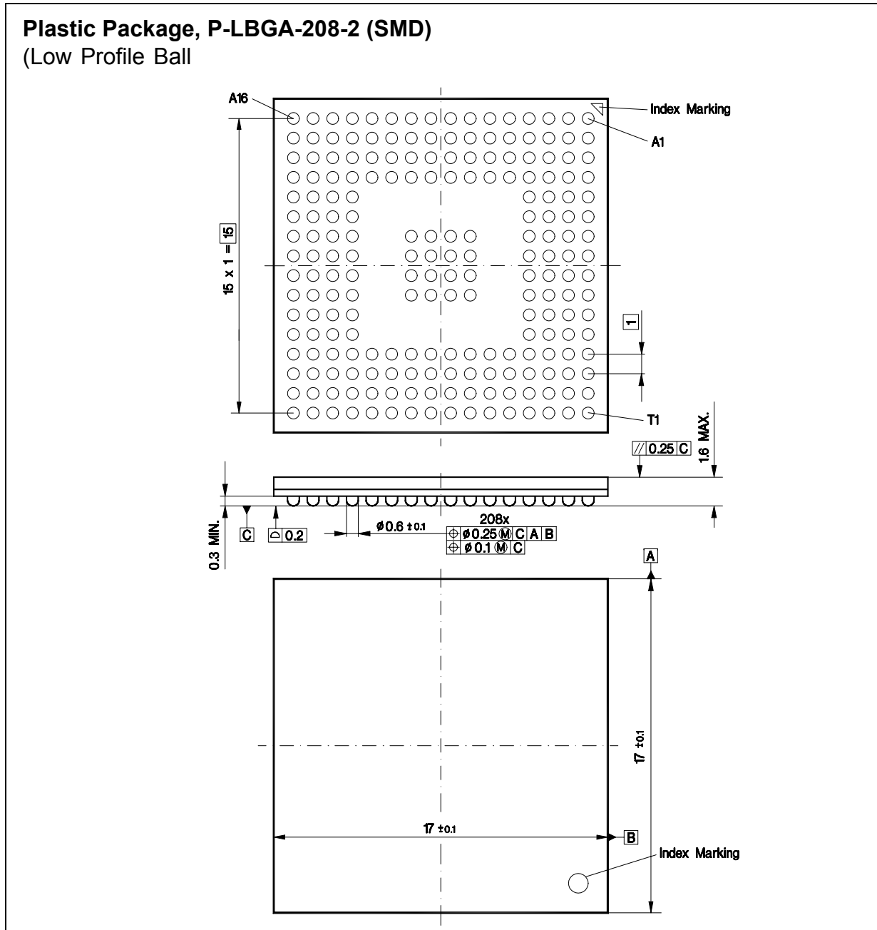
Figure 5-1 P-LBGA-208-2 Package
