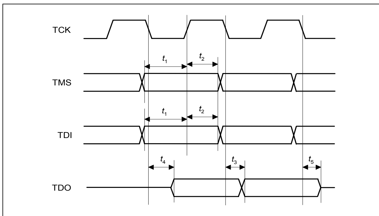
Figure 4-7 JTAG Timing
