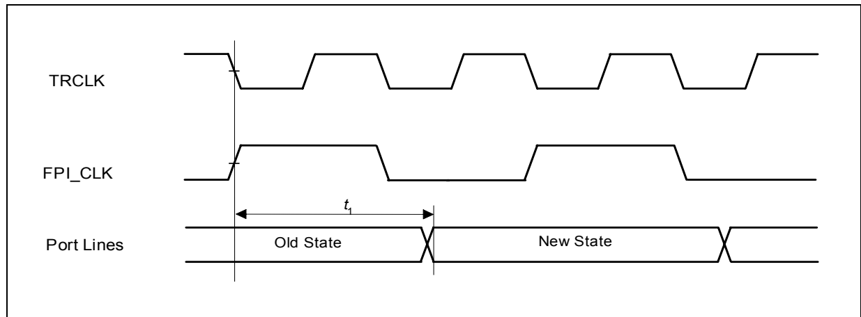
Figure 4-5 Port Timing
