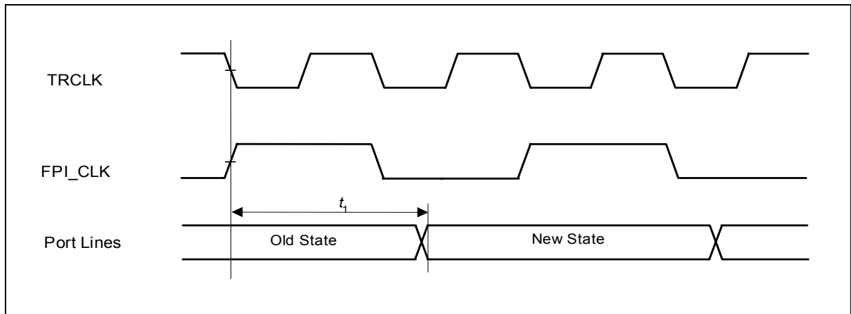
Figure 4-5 Port Timing
