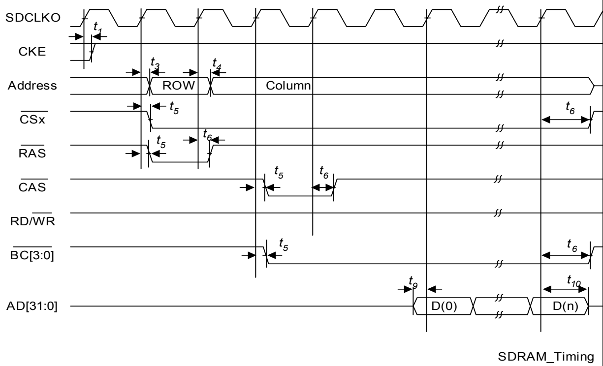
Figure 4-10 SDRAM Access Timing
