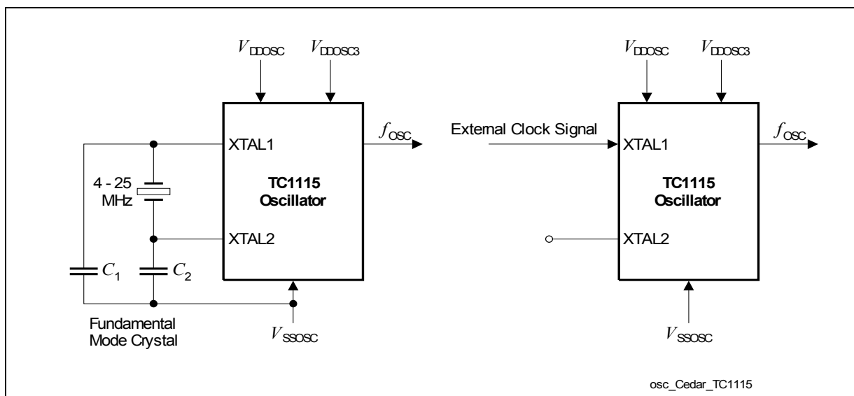
Figure 3-15 Oscillator Circuitries
