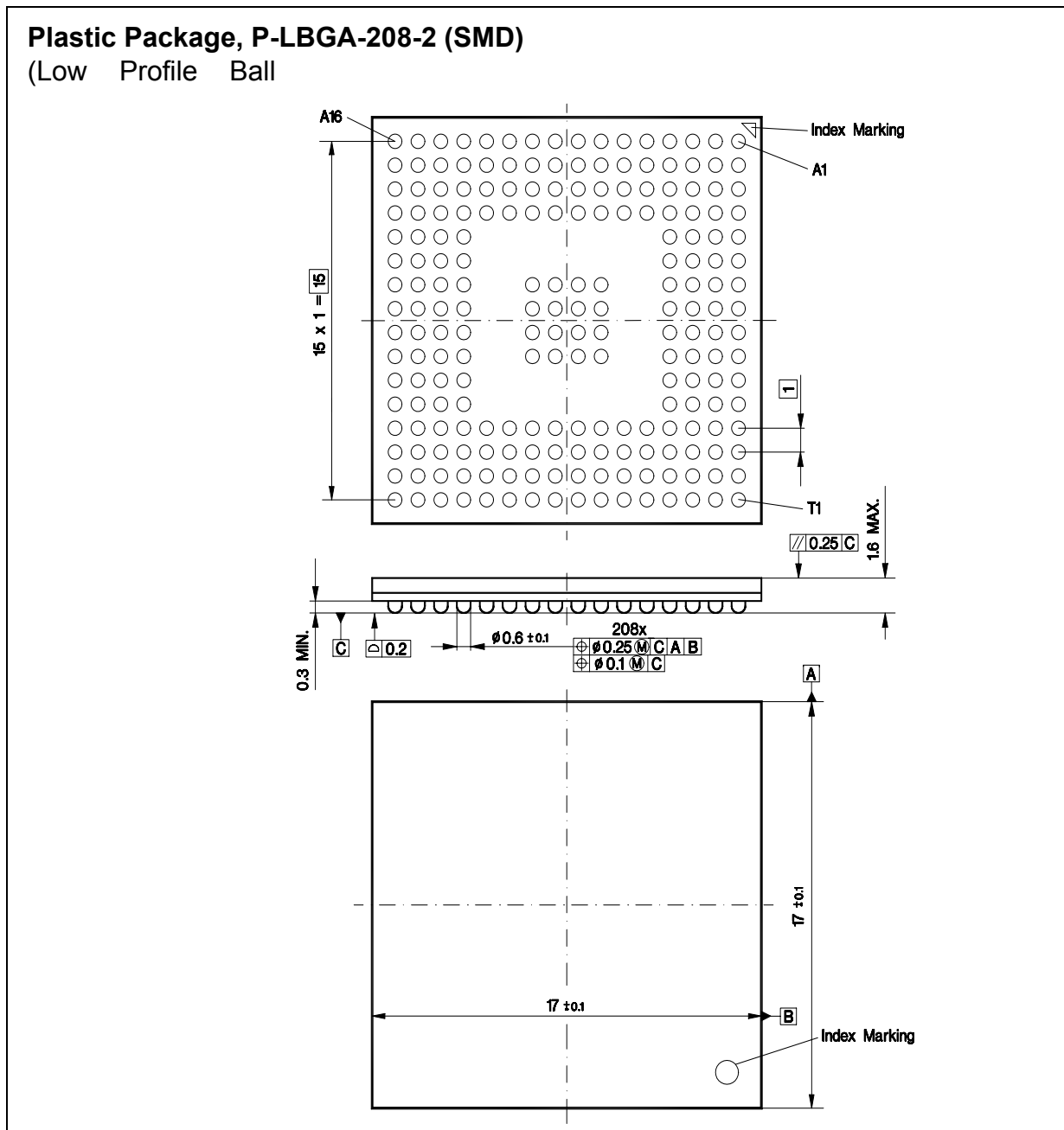
Figure 5-1 P-LBGA-208-2 Package
