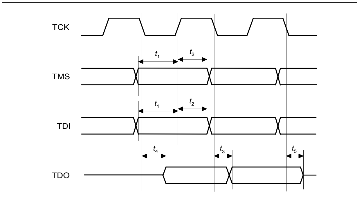
Figure 4-7 JTAG Timing
