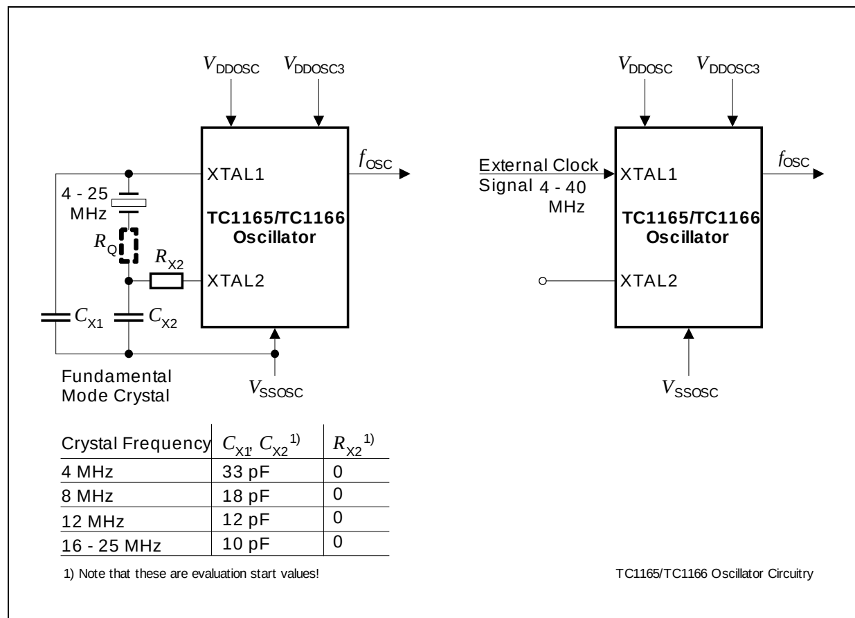
Figure 3-16 Oscillator Circuitries
