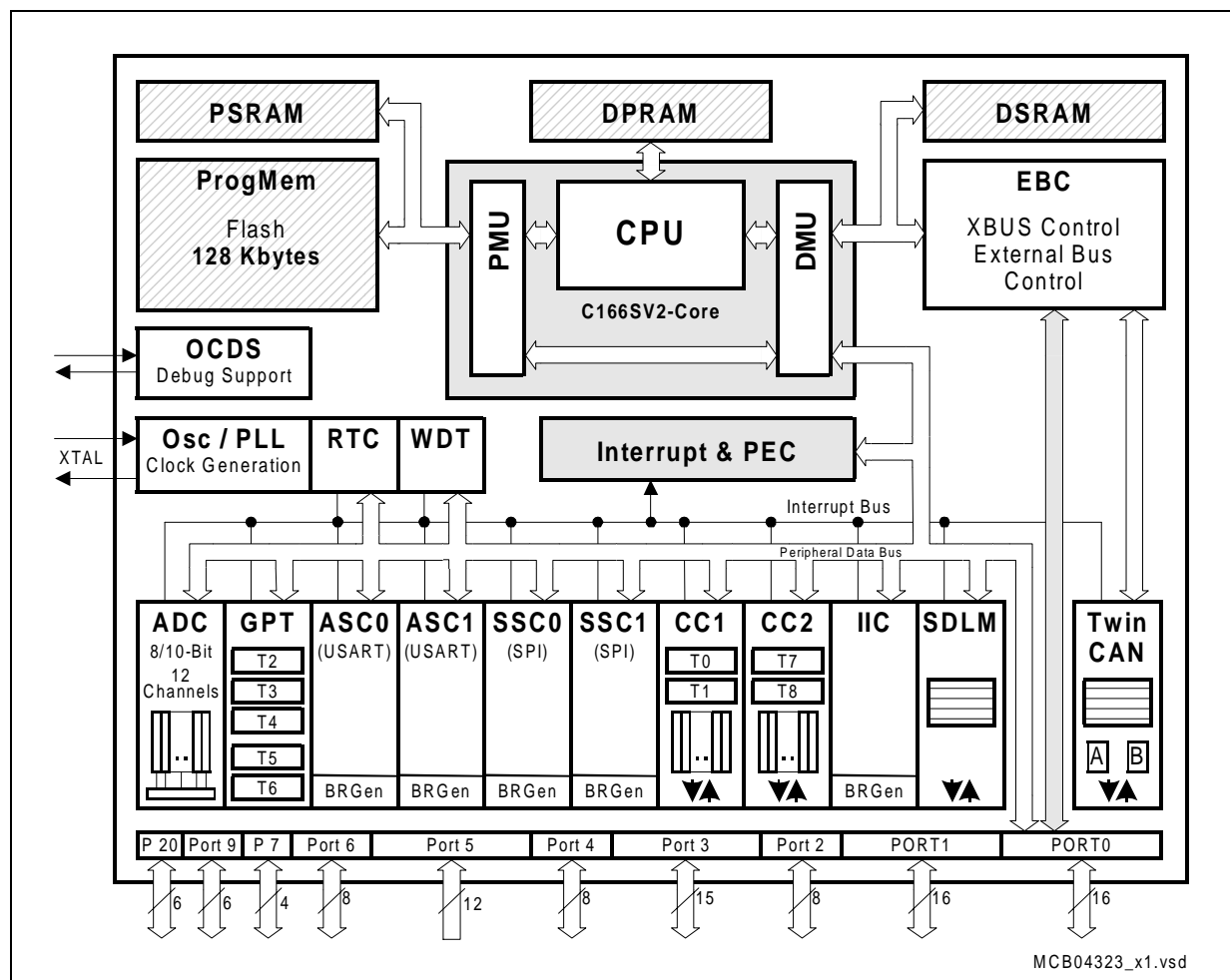
Figure 3 Block Diagram
