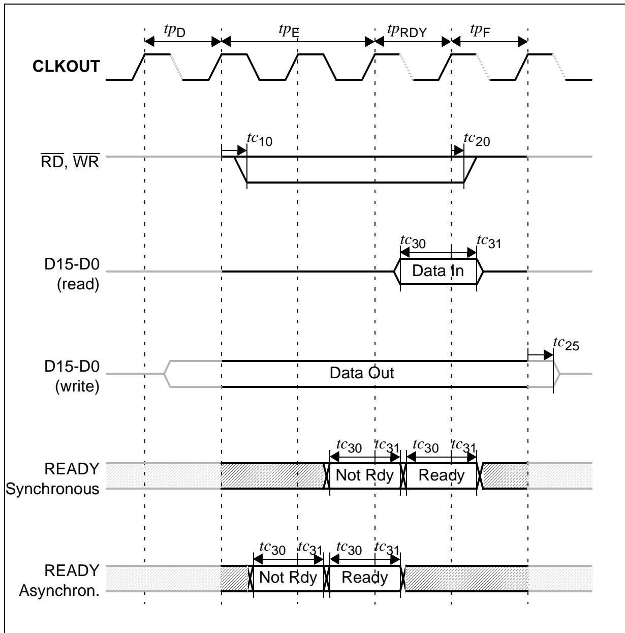
Figure 22 READY Timing
