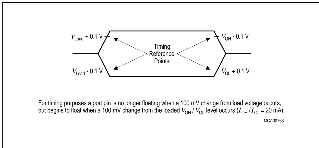
Figure 18 Float Waveforms
