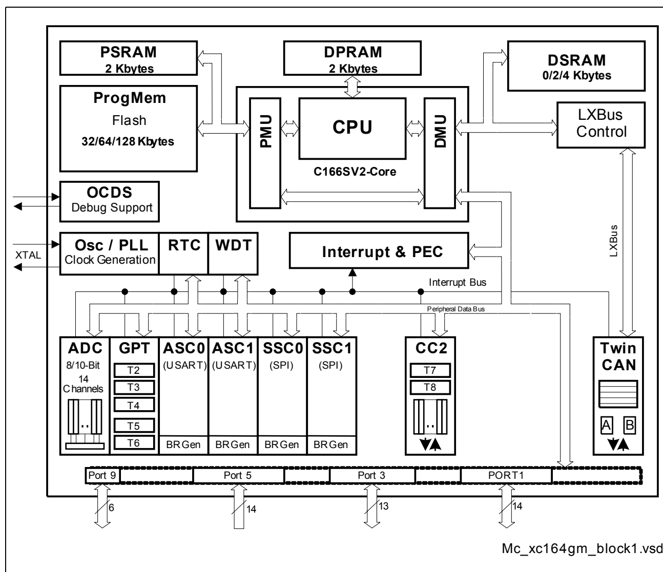
Figure 3 Block Diagram
