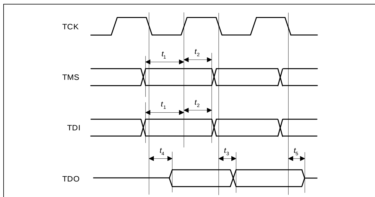
Figure 46 JTAG Timing
