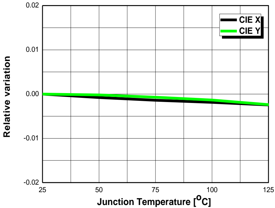
Fig 8. Junction Temperature vs. CIE x, y shift, I_F=40\text{mA} (4200K~6000K)
