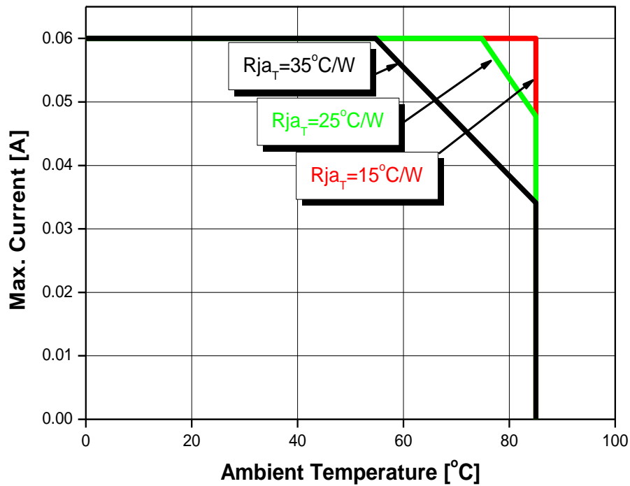
Fig 9. Maximum Forward Current vs. Ambient Temperature, T_{j(max.)}=125^{\circ}\text{C} , I_F=60\text{mA}
