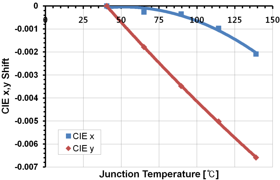
Fig 8. Junction Temperature vs. CIE x,y Shift, I_F=40\text{mA}
