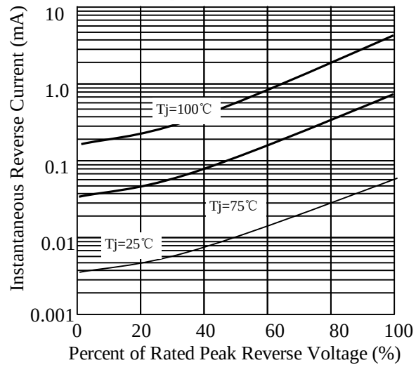
Fig 4. - Typical Reverse Ch. T_J=100^\circ\text{C} ics
