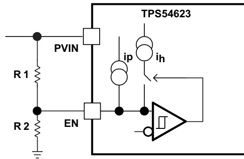
Figure 20. Adjustable PVIN Under Voltage Lock Out, VIN ≥ 4.5V
