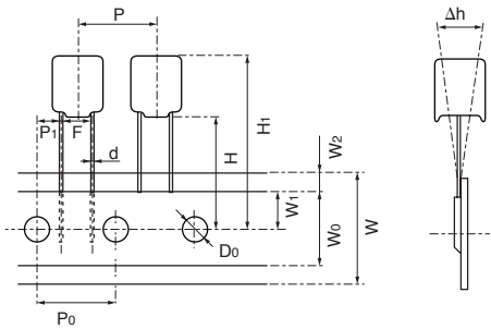
Dimensions of indented square hole plastic tape
