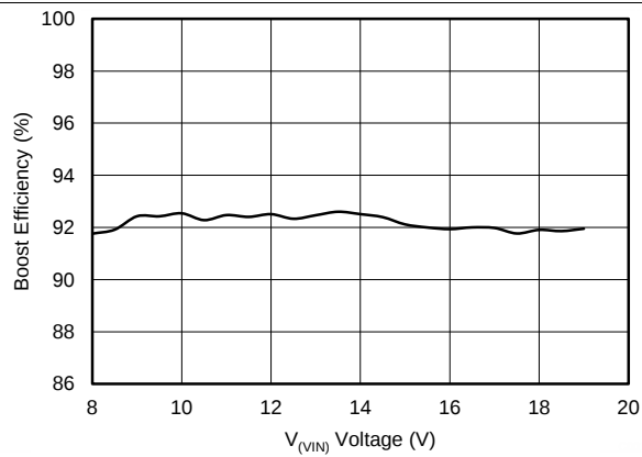
Figure 1. Boost Efficiency vs Input Voltage
