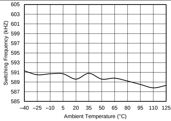
Figure 7. Switching Frequency vs Ambient Temperature
