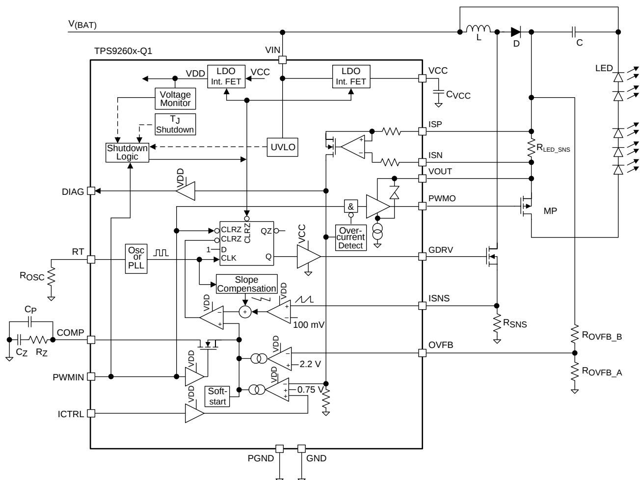
Figure 9. Block Diagram, TPS9260x-Q1 in Boost-To-Battery Configuration
