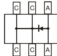
Internal Schematic
