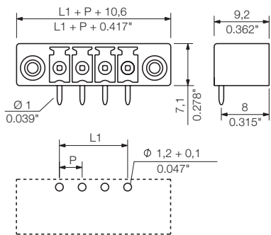
Dimensioned drawing
