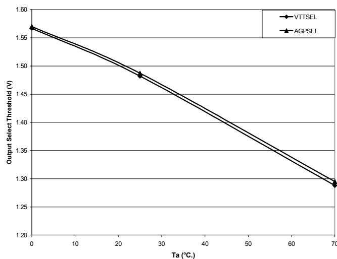
Output Select Threshold vs Ta
