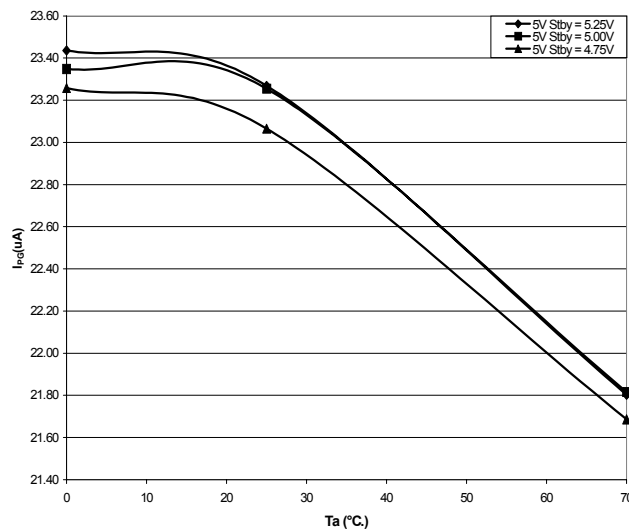
VTT Power Good Source current vs Ta
