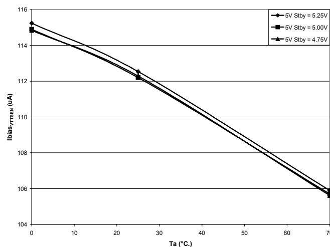
VTT Sense Bias current vs T_a
