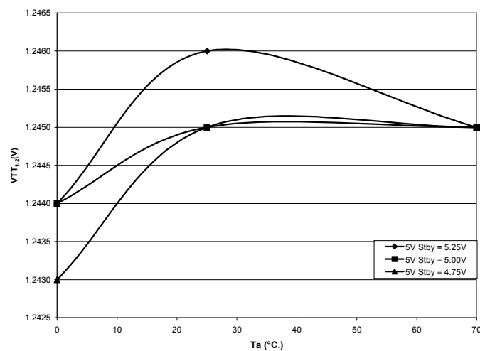
VTT(1.5V) Output Voltage @ I_o = 2A vs T_a
