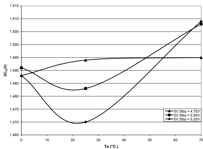
VTT Short circuit Delay Timer Threshold vs Ta
