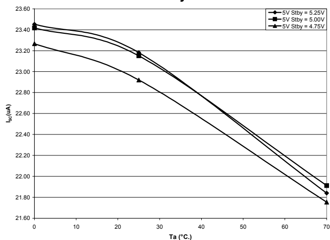
VTT Short circuit Delay source current vs Ta
