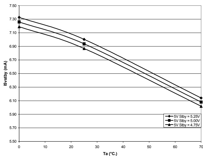
I 5V Stby vs Ta
