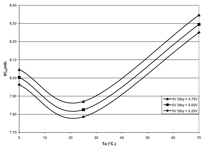
VTT Short circuit Delay Time (Cdelay = 0.1uF) vs Ta
