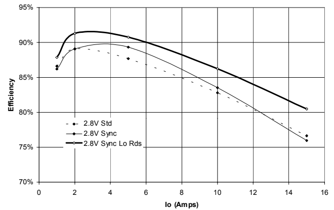
Typical Efficiency at V_o=2.8V
