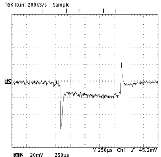
Transient Response V_o=2.8V , I_o=300mA to 10A
