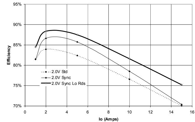
Typical Efficiency at V_o=2.0V
