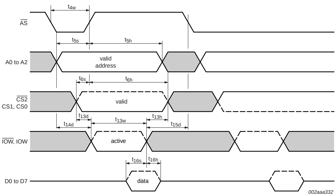
Fig 9. General write timing when using AS signal
