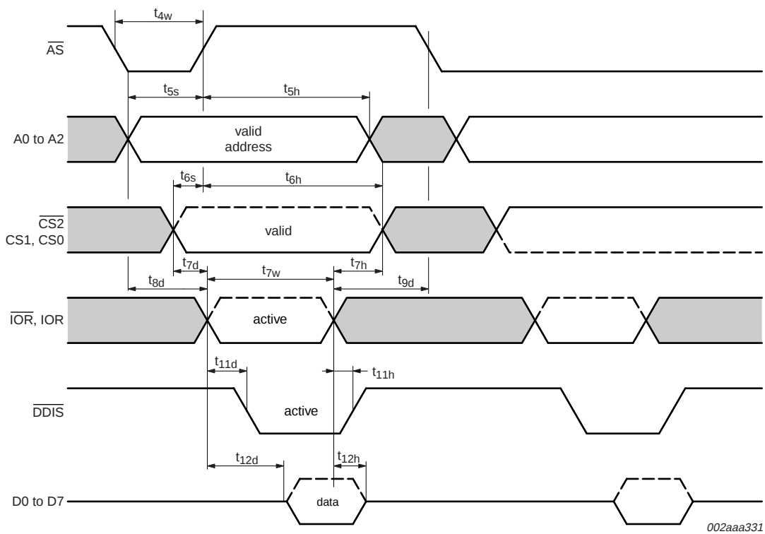
Fig 8. General read timing when using AS signal
