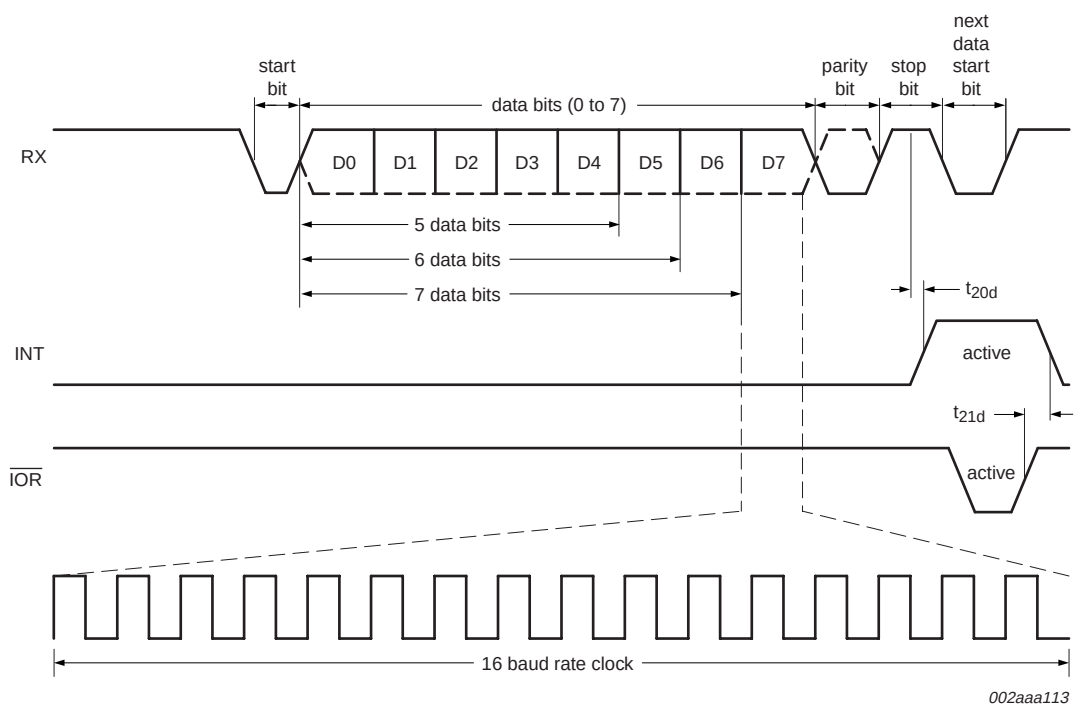
Fig 19. Receive timing
