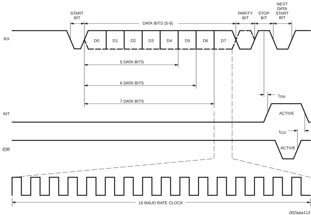
Fig 15. Receive timing.
