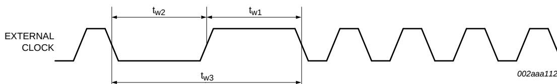
Fig 34. External clock timing
