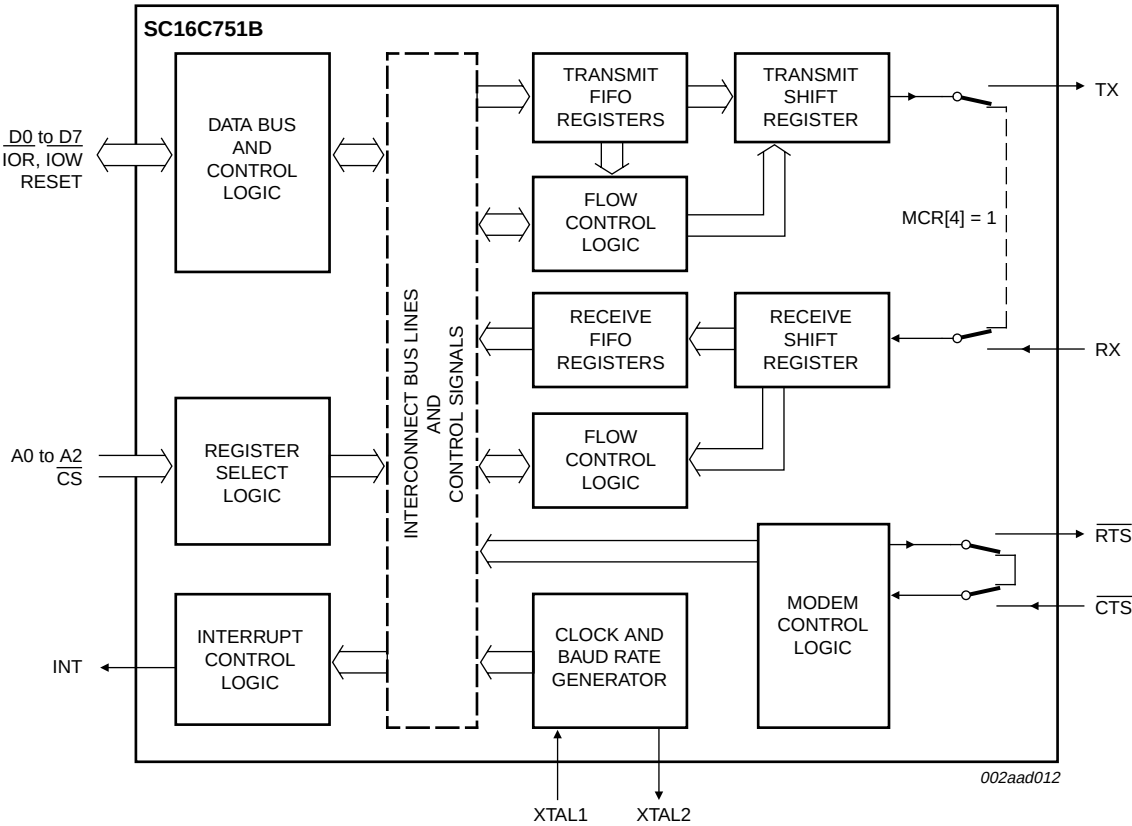
Fig 4. Internal Loopback mode diagram
